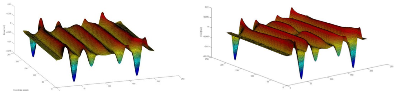
Fig. 5: (left) Finite Element Modeling of a cylindrical, 200 \times 200 mm slumped glass with 1 m curvature radius and 0.4 mm thickness, simulated integration against a paraboloidal integration mould. Spring-back effect is clearly visible (as in Fig. 2) in the space between the ribs. (right) The same simulation with a single piezoceramic element P-876.SP1 by PhysikInstrumente , 16 mm \times 16 mm wide and 0.2 mm thick, fed by a 10 V voltage: the springback effect was corrected locally. FEM performed via the Abaqus® software package (after [23] ).
