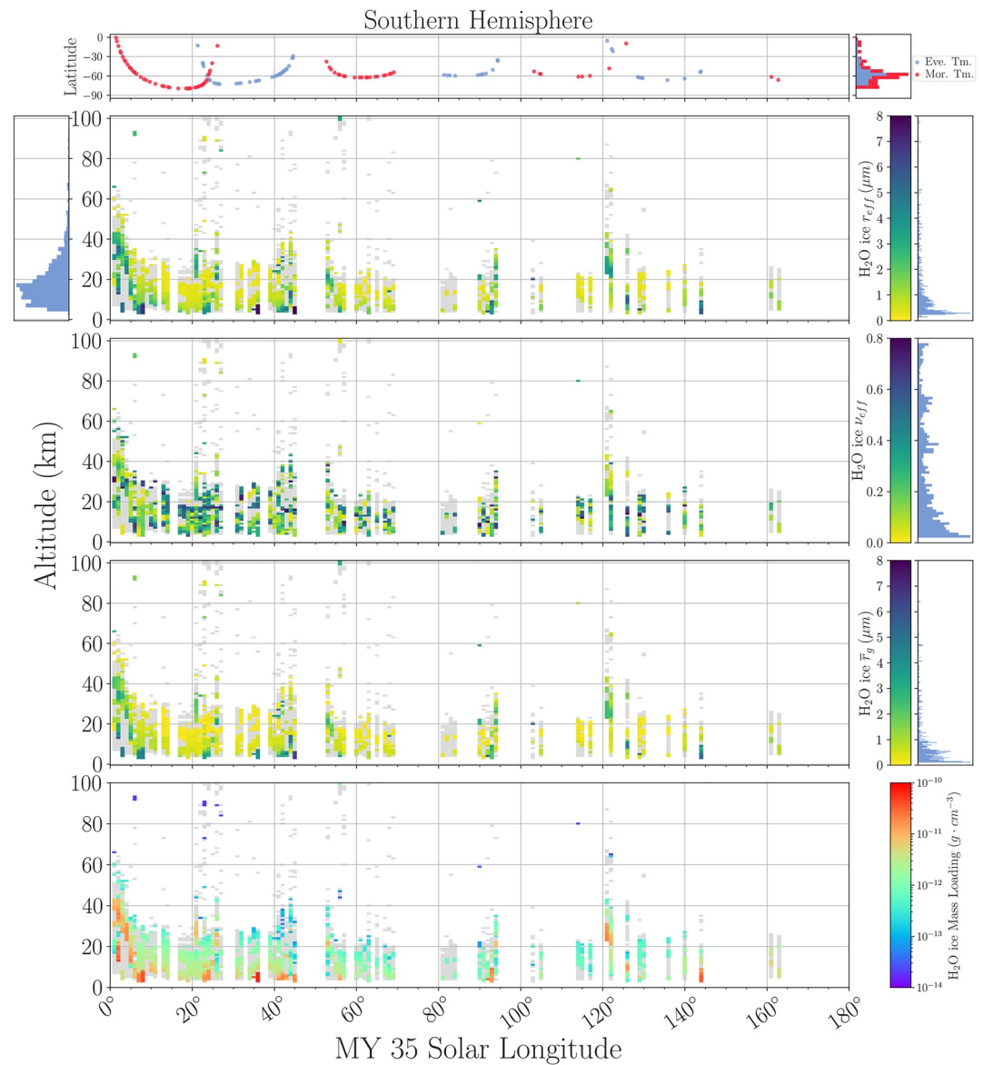
Figure 20. Results of the aerosol distribution properties analysis scheme for \text{H}_2\text{O}_{\text{ice}} in the southern hemisphere during the first half of MY 35. The filtered points (high merit function or low/high effective variance) are shown in light gray. All histograms panels are relative occurrences and share the vertical axis with their relevant parameters.
