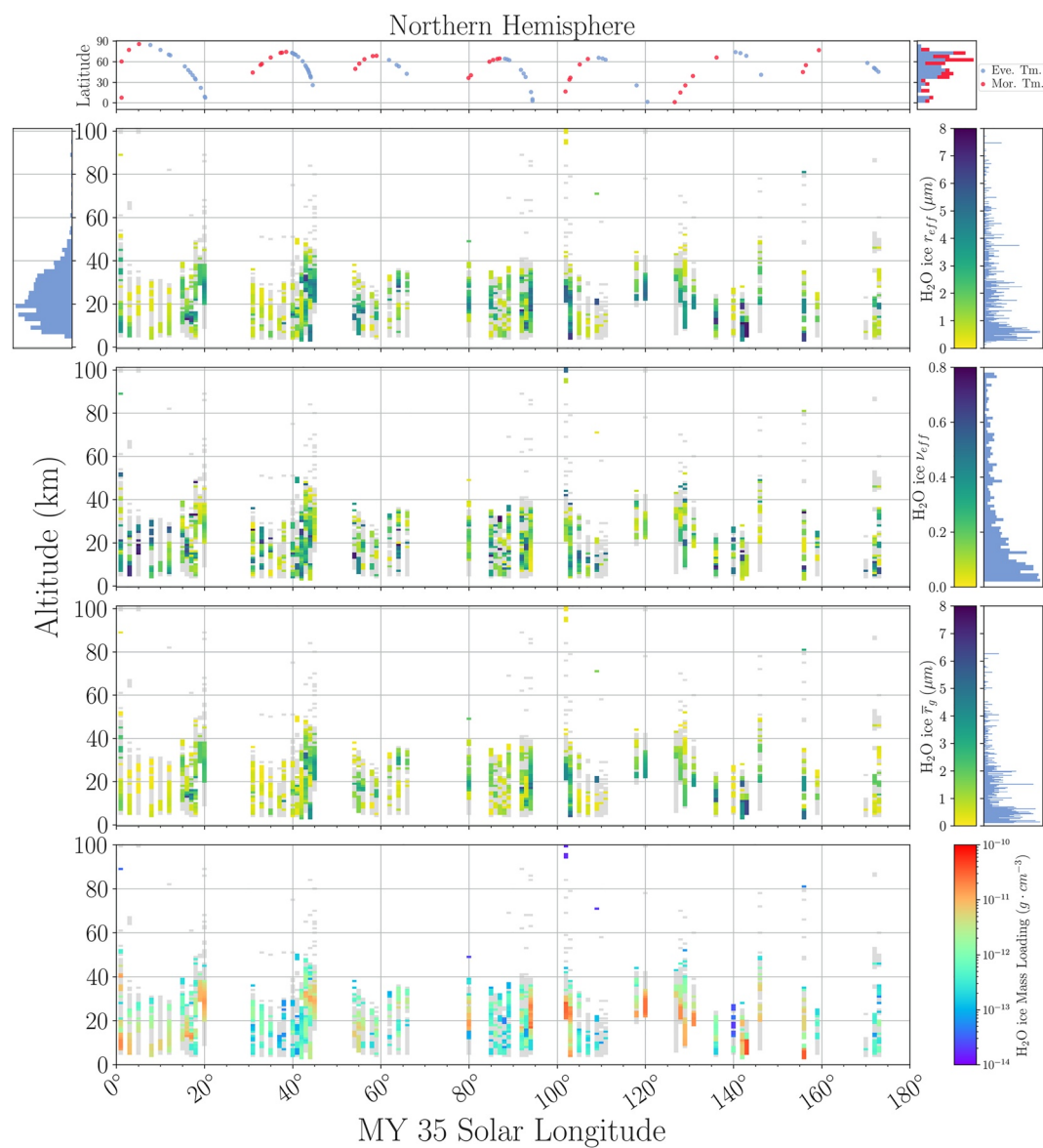
Figure 18. Results of the aerosol distribution properties analysis scheme for \text{H}_2\text{O}_{\text{ice}} in the northern hemisphere during the first half of MY 35. The filtered points (high merit function or low/high effective variance) are shown in light gray). All histograms' panels are relative occurrences and share the vertical axis with their relevant parameters.
