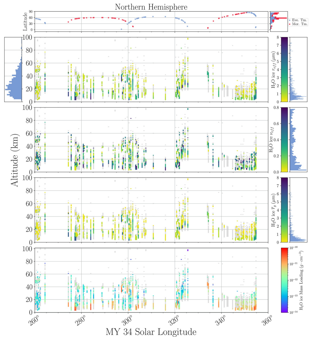
Figure 10. Results of the aerosol distribution properties analysis scheme for \text{H}_2\text{O}_{\text{ice}} in the northern hemisphere during the end of MY34. The filtered points (high merit function or low/high effective variance) are shown in light gray).
