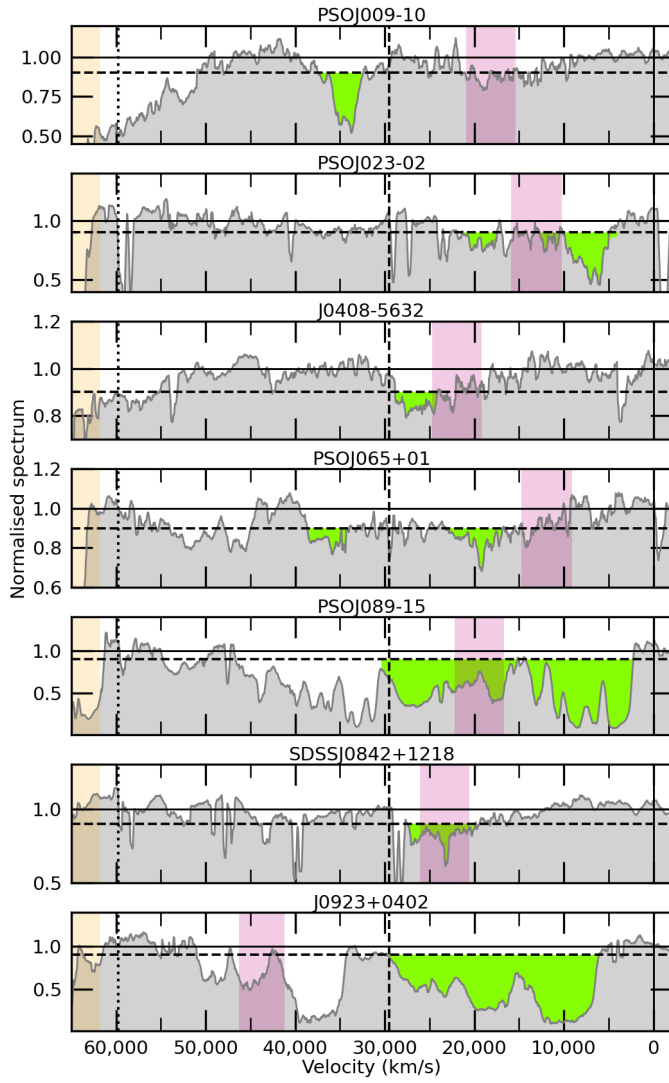
Extended Data Fig. 1 | Normalized spectra of BAL quasars in the XQR-30 sample, smoothed to 500 km/s. The velocity axis in each panel is relative to the rest-frame wavelength of CIV. Vertical solid, dashed, and dotted lines indicate the position of CIV, Si IV and NV, respectively. The horizontal solid (dashed) line represents a flux level of 1.0 (0.9). CIV BALs, corresponding to a flux level of less than 0.9 (equation 1), are highlighted as green shaded areas. We note that the CIV optical depth typically dominates that of Si IV in BAL quasars. This implies that, for example, the BAL feature at v \sim 45000 km/s in PSOJ009-10 cannot be ascribed to a low velocity Si IV BAL because no low velocity CIV BAL with similar velocity is observed in the X-shooter spectrum. The shaded magenta areas indicate the overlapping spectral region between the X-shooter Vis and NIR arms, while orange areas indicate the spectral region affected by substantial intergalactic medium absorption.
