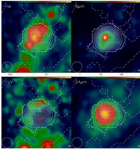
Fig. 1. The CO J=2-1 integrated intensity contours for Francesco’s favorite M33 giant molecular cloud (GMC178) are plotted on maps of H \alpha (upper left panel), GALEX-FUV (lower left panel), Spitzer 8 \mu m (upper right panel) and Spitzer 24 \mu m (lower right panel)
