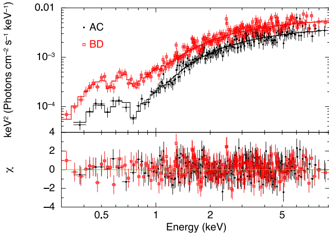
Figure 5. Upper panel: The model including an ionized absorber partially covering the source ( phabs \times (zphabs \times xzpcf \times zpowlw) ) is overplotted on the low- (AC) and high-state (BD) unfolded spectra of Mrk 915. Lower panel: Relevant residuals, plotted in terms of sigmas with error bars of size one.
