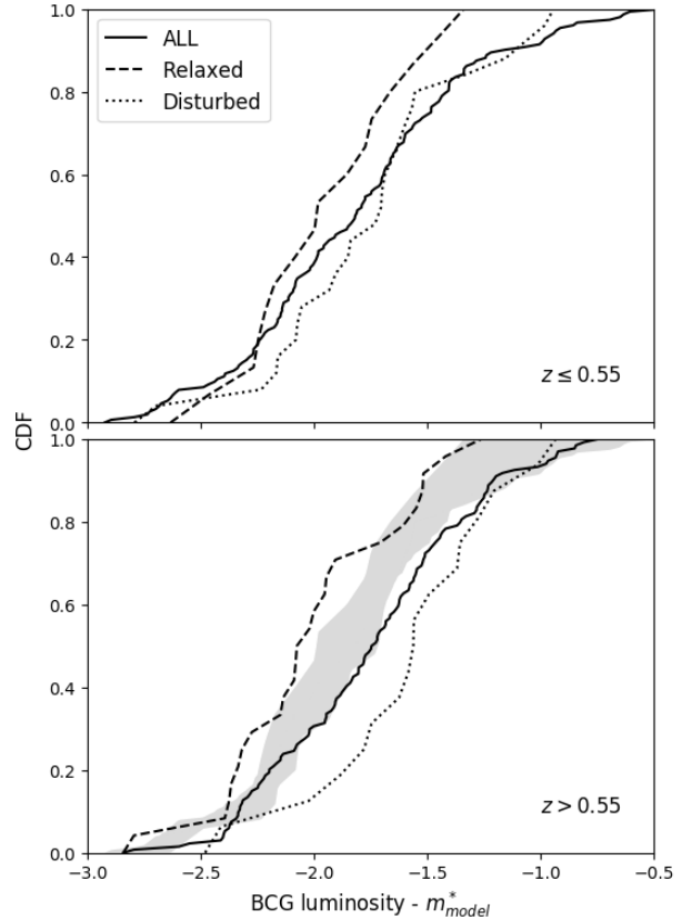
Figure 4. Cumulative distribution of the BCG luminosity ( r -band at z < 0.35 , i -band at z < 0.7 , and z -band at z > 0.7 ) for the total (solid line), relaxed (dashed line), and disturbed (dotted line) cluster samples. Top panel: BCGs at z \leq 0.55 . Bottom panel: BCGs at z > 0.55 . Shaded area corresponds to the area covered by the BCG distributions at the low redshift bin.
