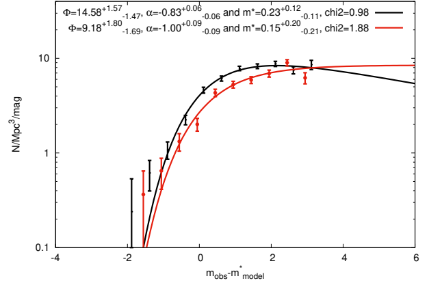
Figure 9. Stacked luminosity functions for the disturbed (red) and relaxed (black) sample, within 0.5 \times r_{200} , including all cluster galaxies. We use the m^* model and the band redwards the 4000Å break to offset all LFs to the same photometric frame
