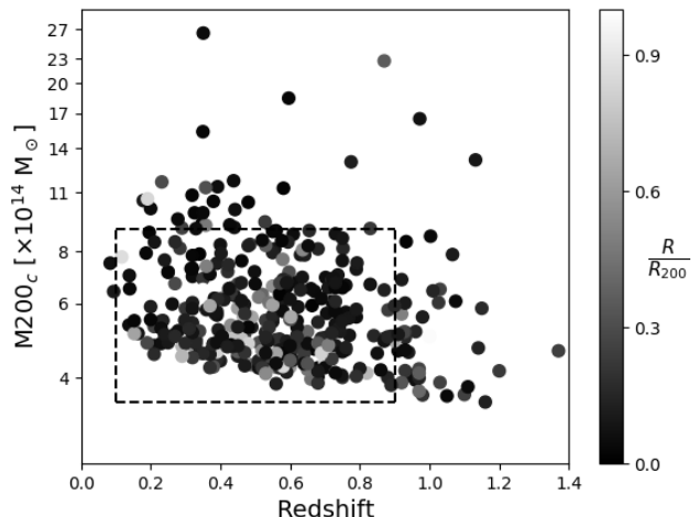
Figure 1. The mass redshift distribution of 368 SPT clusters imaged with DES Y3 data. The dashed box corresponds to limits applied to the SPT-SZ sample to select our sample. In light gray clusters with larger BCG to SZ centroid offset ( D_{\text{BCG-SZ}} ) while the dark points correspond to systems with lower D_{\text{BCG-SZ}} .
