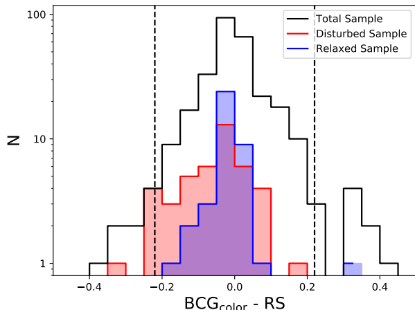
Figure 5. BCG color for the total, the relaxed, and the disturbed cluster samples with respect to the red sequence (as defined in § 2.4). The BCG colors, and m^* , are estimated depending on the cluster redshift; g-r at z < 0.35 , r-i at z < 0.7 , and i-z at z > 0.7 . Vertical lines are at \pm 0.22 mags, corresponding to our 3\sigma red-sequence width (López-Cruz et al. 2004).
