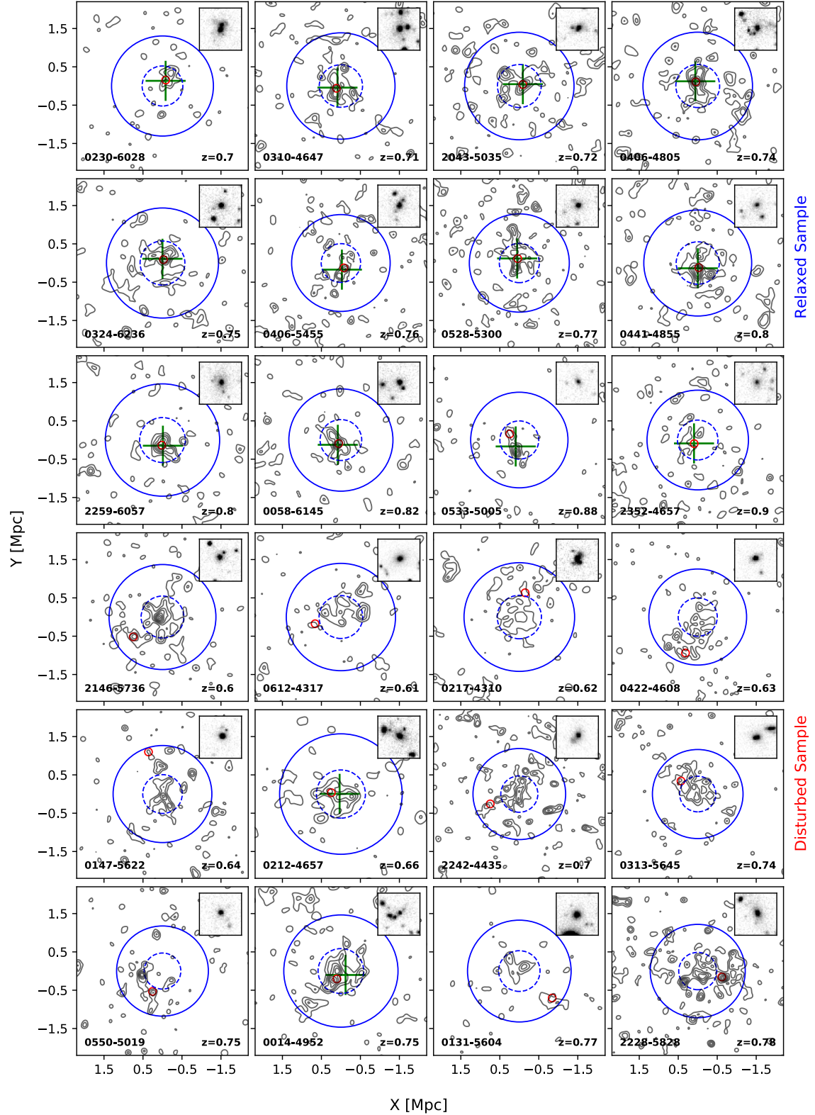
Figure 13. The top 12 clusters correspond to the highest redshift relaxed systems. The outer circled represents r_{200} , while the inner circle corresponds to 0.4r_{200} . Contours correspond to the red sequence galaxy distribution. The green cross shows the X-ray peak emission while i -band images of the BCG is shown in the top right corner. The relaxed systems are selected if the BCG is within 42/71 kpc of the X-ray peak/centroid (Mann & Ebeling 2012), if K_0 < 30 \text{ keV cm}^2 (McDonald et al. 2013), or if it is classified as relaxed by its morphology with a A_{\text{phot}} \leq 0.1 (Nurgaliev et al. 2017). The bottom 12 clusters correspond to the highest redshift disturbed systems centered in the SZ emission. Most of the clusters have been selected by the large displacement of the BCG with respect to SZ center of X-ray peak/center, while a fraction relies on a gas morphology index A_{\text{phot}} . In the latter case the BCG is not necessarily significantly displaced from the gas center, as shown by SPT-CLJ0014-4952.
