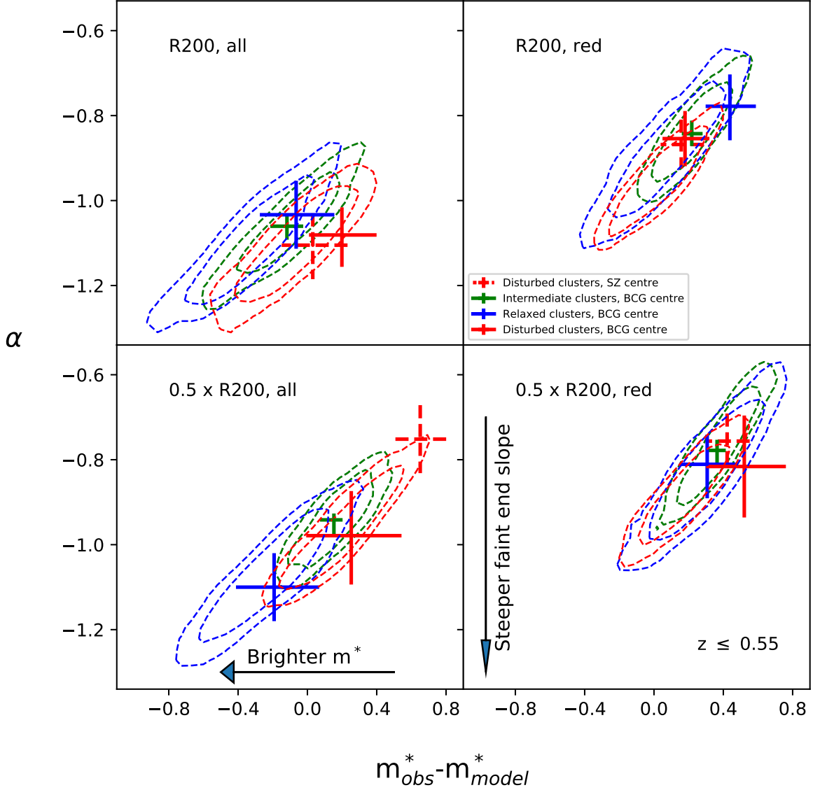
Figure 11. \alpha - \Delta m^*(m_{obs}^* - m_{model}^*) for cluster galaxies (all) and red sequence galaxies (red), within 1 and 0.5 r_{200} , at z \leq 0.55 . We obtain m_{obs}^* by fitting the data, while m_{model}^* corresponds to the model as discussed in § 2.4. Solid red crosses represent disturbed clusters using the BCG as a center (26 clusters), dash red crosses represent disturbed clusters using the SZ centroid as a center, blue crosses correspond to the relaxed sample (16 clusters) while green crosses correspond to the intermediate sample (see § 4.1.3 for details; 111 clusters), both using the BCG as a center. Dashed red/blue contours correspond to 68% and 90% of the fits, when the center is randomized 600 times within 0.4-1 r_{200} of the SZ center, for the disturbed/relaxed sample. Green contours correspond to 68% and 90% of the fits, obtained by stacking 26 randomly selected clusters from the intermediate cluster sample, using the BCG as a center 600 times. At this redshift range all cluster populations seems to occupy a very similar \alpha - \Delta m^* parameter space.
