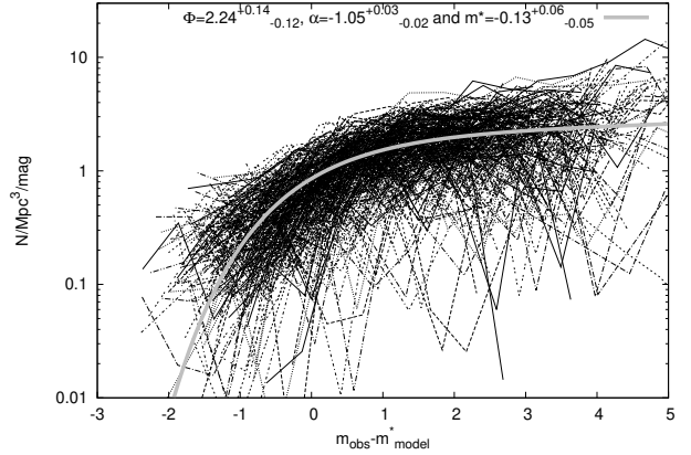
Figure 8. Luminosity functions of individual clusters for the all population up to their completeness limit. We use the m^* model and the band redwards the 4000\text{\AA} break to offset all LFs to the same photometric rest-frame. The stacked result (gray solid line) is created using individual LFs up to m^* + 3 , or the individual completeness limit if m^* + 3 can not be reached.
