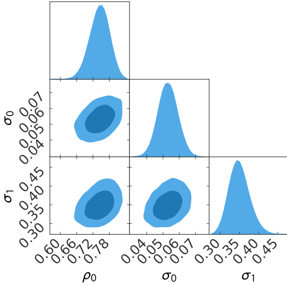
Figure 7. 1\sigma and 2\sigma solutions of the three parameter model of equation 5 that describes the D_{\text{BCG-SZ}} distribution.
