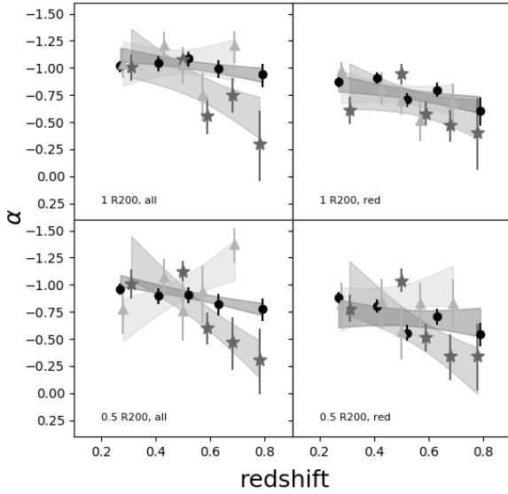
Figure 10. Faint end \alpha evolution for the disturbed sample (triangles), the relaxed sample (stars), and all clusters excluding the disturbed and relaxed sample (dots). The shaded areas correspond to 1\sigma contours.
