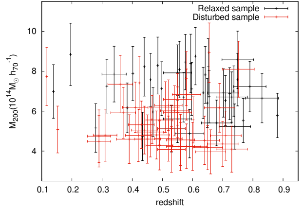
Figure 3. The location of relaxed (41) and disturbed (43) cluster sample mass-redshift plane. The mass and redshift cuts described in section § 2.3 have been applied. It can be seen that the average mass of the relaxed clusters are higher than the average mass of the disturbed clusters.
