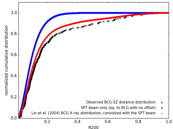
Figure 6. The full cluster sample cumulative central offset distribution (black), D_{\text{BCG-SZ}} compared to an X-ray sample from the literature (red) and the case of pure SPT positional uncertainty (blue).
