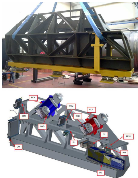
Fig. 1. Opto-mechanics of the ESPRESSO spectrograph. Top: optical bench as of July 2015. Bottom: scheme (APSU: Anamorphic Pupil-Slicer Unit, BCA: Blue Camera, BTM: Blue Transfer Mirror, BXD: Blue Cross-Disperser, CM: Main Collimator, DC: Dichroic, EG: Echelle Grating, FL: Field Lens, PM: Field Mirror, RCA: Red Camera, RTM: Red Transfer Mirror, RXD: Red Cross-Disperser).
