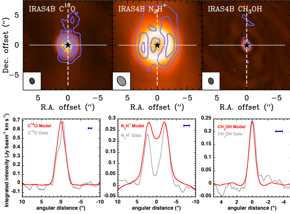
Fig. 2. Top row: Comparison of the observations (contours) with the synthetic maps (colour background) produced by the best fit model for IRAS4B with E_b(\text{CO}) = 1200 K and E_b(\text{N}_2) = 1000 K. Top left: \text{C}^{18}\text{O} (2–1), centre: \text{N}_2\text{H}^+ (1–0), right: \text{CH}_3\text{OH} (5 1 –4 2 ), integration intervals are the same as in Fig. 1, while the contour spacing is in steps of 3\sigma , starting at 3\sigma . The white dashed lines show the outflow direction, while the dotted lines show the direction of the intensity cuts. The scaling of the maps can be understood in comparison with the cuts in the bottom row. Bottom row: Cuts perpendicular to the outflow direction (P.A. = 0^\circ ) for \text{C}^{18}\text{O} , \text{N}_2\text{H}^+ , and \text{CH}_3\text{OH} (left to right). Grey lines show the data, red lines the model. The blue bars in the top right corners of the bottom panels show the HPBW along the cut.
