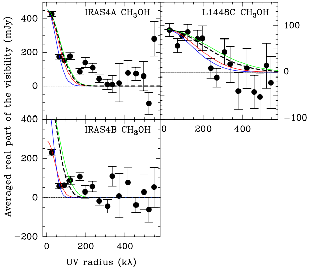
Fig. B.2. Same as Figure B.1, but for \text{CH}_3\text{OH} in IRAS4A (top left), L1448C (top right), and IRAS4B (bottom left). The data is radially averaged in bins of 50 m with task uv_circle in MAPPING. The parameters of the fits are listed in Table 4.
