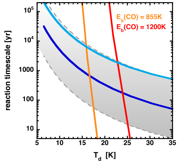
Fig. 7. CO ice depletion timescale (dark blue line) and thermal desorption timescales for binding energies of 855 K (orange line) and 1200 K (red line) as function of the dust temperature for the density profiles of IRAS4B. The light blue line shows the free-fall time for an enclosed mass of 0.5 M_{\odot} . The points of intersection at \sim 17 K and \sim 24 K mark the locations of the CO snow line for the two different values of the binding energy. The grey area shows the range of depletion timescales if the dust density is varied by a factor of ten. For a binding energy of 855 K, the variation of the density translates into a variation of the snow line location at \sim 16 K or \sim 17 K, while for a binding energy of 1200 K, the modified snow line locations would be at \sim 23 K or \sim 25 K.
