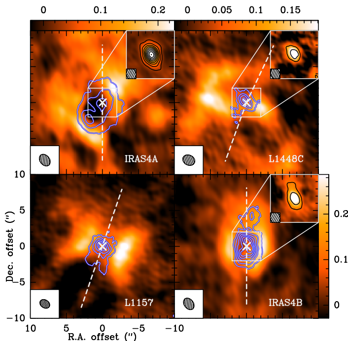
Fig. 1. Anticorrelation between \text{N}_2\text{H}^+ and \text{C}^{18}\text{O} . Colour background: \text{N}_2\text{H}^+ (1–0) emission integrated over all seven hyperfine components. The noise in these maps is \sigma=(0.030, 0.027, 0.025, 0.029) \text{Jy beam}^{-1} \text{ km s}^{-1} for IRAS4A, L1448C, L1157, and IRAS4B, respectively. The wedges show the \text{N}_2\text{H}^+ intensity scale in \text{Jy beam}^{-1} \text{ km s}^{-1} . For the two lower panels the scaling is the same. Contours show emission of \text{C}^{18}\text{O} (2–1) in steps of 6\sigma (IRAS4A and 4B) or 3\sigma (L1448C and L1157), starting at 3\sigma , with \sigma=(0.044, 0.029, 0.031, 0.033) \text{Jy beam}^{-1} \text{ km s}^{-1} for IRAS4A, L1448C, L1157, and IRAS4B, respectively. The inlays in the upper right corners show the methanol emission as colour background and contours in steps of 3\sigma , starting at 3\sigma inside the central 2'' , with \sigma=(0.028, 0.019, 0.027) \text{Jy beam}^{-1} \text{ km s}^{-1} for IRAS4A, L1448C, and IRAS4B. In L1157, the methanol line has not been detected at a 3\sigma level. The filled ellipses in the lower left corner of the panels indicate the synthesized beam sizes of the \text{N}_2\text{H}^+ observations at 3 mm. The dashed white lines illustrate the small-scale outflow directions (see Table 3 and Section 3.1) and the white crosses show the positions of the sources as listed in Table 1.
