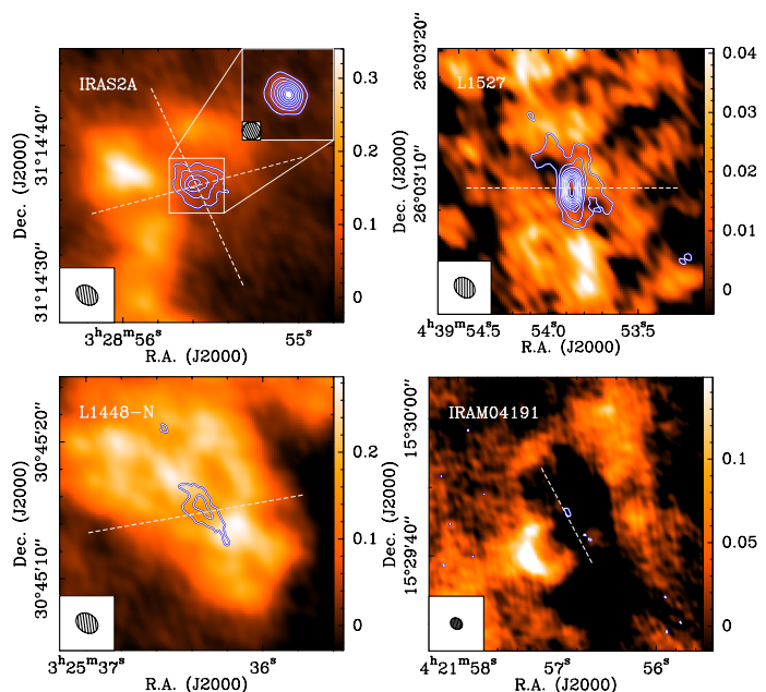
Fig. A.1. \text{N}_2\text{H}^+ and \text{C}^{18}\text{O} integrated intensity maps for IRAS2A (top left), L1527 (top right), L1448-N (bottom left), and IRAM04191 (bottom right) as prototypical sources for the four morphology classes we find in the full sample of sources. Colour background: \text{N}_2\text{H}^+ (1–0) emission integrated over all seven hyperfine components. The noise in these maps is \sigma = (0.043, 0.012, 0.033, 0.032) Jy beam ^{-1} km s ^{-1} for IRAS2A, L1527, L1448-N, and IRAM04191, respectively. The wedges show the \text{N}_2\text{H}^+ intensity scale in Jy beam ^{-1} km s ^{-1} . Note that while for the first three sources the FOV is 20'' \times 20'' , it is 40'' \times 40'' for IRAM04191 in order to show the full ring-like morphology. Contours show integrated emission of \text{C}^{18}\text{O} (2–1) in steps of 3\sigma , starting at 3\sigma up to 60\sigma , with \sigma = (0.037, 0.022, 0.038, 0.018) Jy beam ^{-1} km s ^{-1} for IRAS2A, L1527, L1448-N, and IRAM04191, respectively. The \text{C}^{18}\text{O} emission was integrated over \pm 3 km s ^{-1} around the systemic velocity of each source. The inset in the upper right corners of the top left panel shows the methanol emission towards IRAS2A as colour background and contours in steps of 3\sigma , starting at 3\sigma up to 60\sigma inside the central 2'' . The filled ellipses in the lower left corner of the panels indicate the synthesized beam sizes of the \text{N}_2\text{H}^+ observations at 3 mm. The dashed white lines illustrate the small-scale outflow directions (cf. Codella et al. 2014, Hogerheijde et al. 1998, Podio et al. in prep., Belloche et al. 2002).
