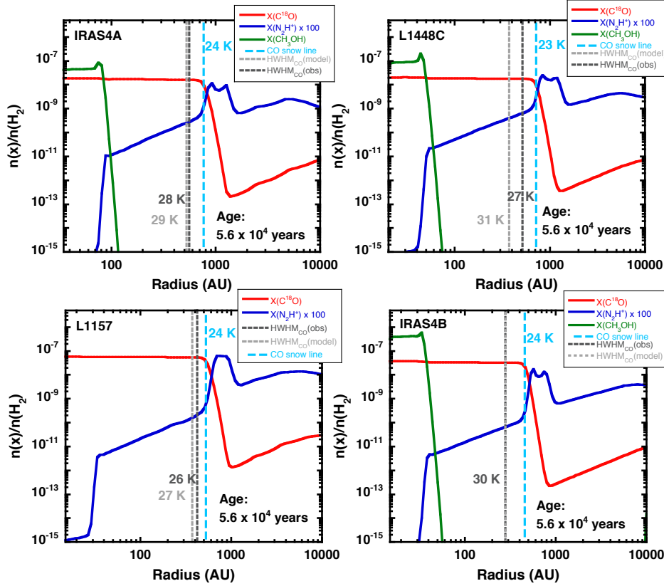
Fig. 3. Fractional chemical abundances, relative to \text{H}_2 , of \text{C}^{18}\text{O} (red lines), \text{N}_2\text{H}^+ (blue lines), and \text{CH}_3\text{OH} (green lines), computed by Astrochem for the envelope structures of IRAS4A (top left), L1448C (top right), L1157 (bottom left), and IRAS4B (bottom right). The light grey dotted lines show the HWHM of the modelled emission, the dark grey dotted lines the HWHM of the observed emission in \text{C}^{18}\text{O} (see Table 3), while the light blue dashed line shows the location of the CO snow line in the model (see Table 5). The figure also indicates the dust temperature values at the respective radii. In IRAS4B, the observed and modelled HWHM are the same.
