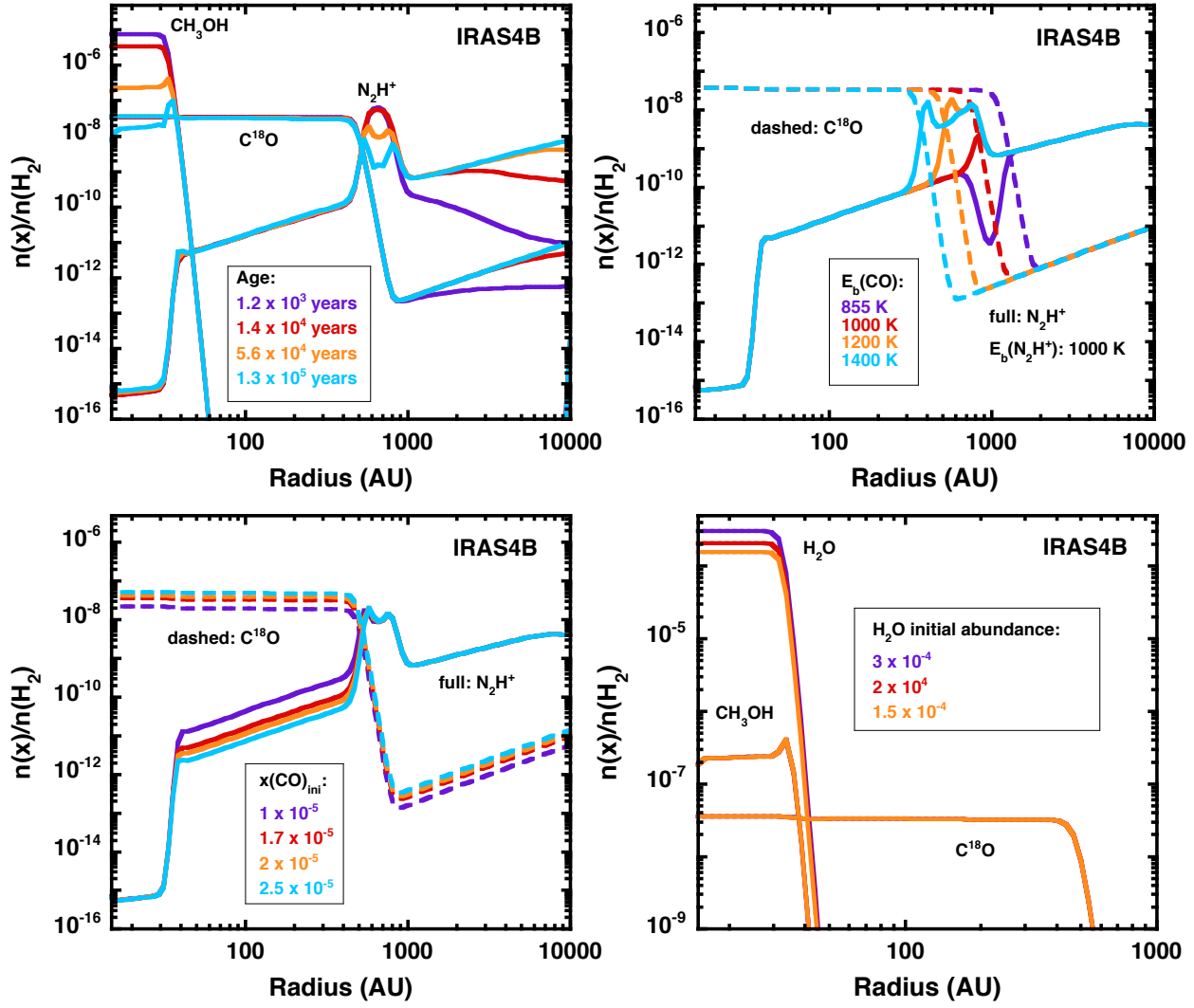
Fig. C.1. Dependences of the chemical model on various free parameters. Top left: The fractional abundances of CH_3OH , C^{18}O , and N_2H^+ are shown for four different chemical ages. Same colours identify abundance curves at the same chemical time for chemical ages as indicated in the legend. Top right: The fractional abundances of C^{18}O (dashed lines) and N_2H^+ (full lines) are displayed for different values of the CO binding energy. Same colours identify abundance curves computed with the same CO binding energy as indicated in the legend. Bottom left: The fractional abundances of C^{18}O (dashed lines) and N_2H^+ (full lines) are displayed for different values of the initial fractional CO abundance. Same colours identify abundance curves computed with the same CO initial abundance as indicated in the legend. Bottom right: The fractional abundances of H_2O , CH_3OH , and C^{18}O are shown for four different values of the initial fractional H_2O abundance. Same colours identify abundance curves computed with the same H_2O initial abundance as indicated in the legend.
