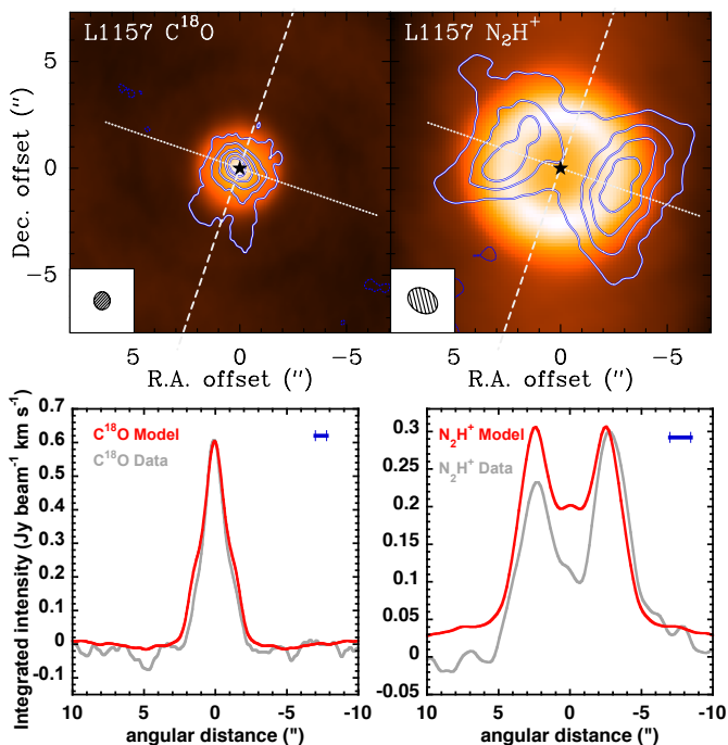
Fig. 6. Same as Fig. 2, but without methanol, for L1157. The cuts are performed at a P.A. of 71^\circ , perpendicular to the outflow direction (P.A. = 161^\circ ).
