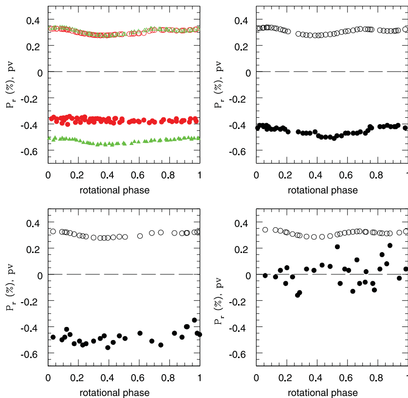
Figure 3. The ‘polarimetric light curves’ used in the present analysis, namely the plots of P_r versus the computed rotational phase at each epoch of measurement (full symbols). Each plot shows also the average albedo of the region of the Vesta’s surface visible at the corresponding epochs of observation, plotted against the corresponding rotational phase (open symbols). The albedo values show a sinusoidal variation around a value of about 0.30. Top-left: 1977 (red) and 1978 (green) data. Top-right: 1986 data. Bottom-left: 1988 data. Bottom-right: 2011 data. Note that we plot the P_r parameter, namely the fraction of linear polarization with sign, and that nearly all the measurement were taken at phase angles corresponding to negative polarization. The general trend is an increasing of polarization for decreasing albedo, apart from the noisy 2011 data, which were taken close to the inversion angle, when the degree of polarization was close to zero.
