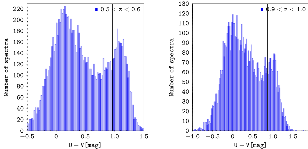
Figure 4. Rest-frame U - V colour distribution for VIPERS galaxies in the redshift bin 0.5 < z < 0.6 (left panel) and 0.9 < z < 1.0 (right panel). The vertical solid lines indicate the adopted separation for red early-type galaxies and blue late-type galaxies, defined by an evolving cut [19].
