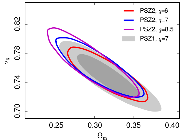
Fig. 3: Contours at 95 % for different signal-to-noise thresholds, q = 8.5, 7 , and 6 , applied to the 2015 MMF3 cosmology sample for the SZ+BAO+BBN data set. The contours are compatible with the 2013 constraints ( Planck Collaboration XX 2014 ), shown as the filled, light grey ellipses at 68 and 95 % (for the BAO and BBN priors of Sect 5.2; see text). The 2015 catalogue thresholded at q > 8.5 has a similar number of clusters (190) as the 2013 catalogue (189). This comparison is made using the analytical error-function model for completeness and adopts the reference observable-mass scaling relation of the 2013 analysis ( 1 - b = 0.8 , see text). The redshift distributions of the best-fit models are shown in Fig. 4. For this figure and Fig. 4, we use the one-dimensional likelihood over the redshift distribution, dN/dz (Eq. 4).
