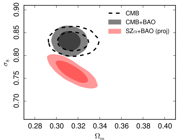
Fig. 13: Prediction of cluster constraints with a possible future mass bias prior of 1 - b = 0.78 \pm 0.01 . The black shaded region and dashed contours reproduce the current primary CMB and primary CMB+BAO constraints from Planck for the base \Lambda CDM model. The red shaded contours present the constraints expected from this mass bias prior applied to the present Planck cluster cosmology sample with the SZ+BAO+BBN data set.
