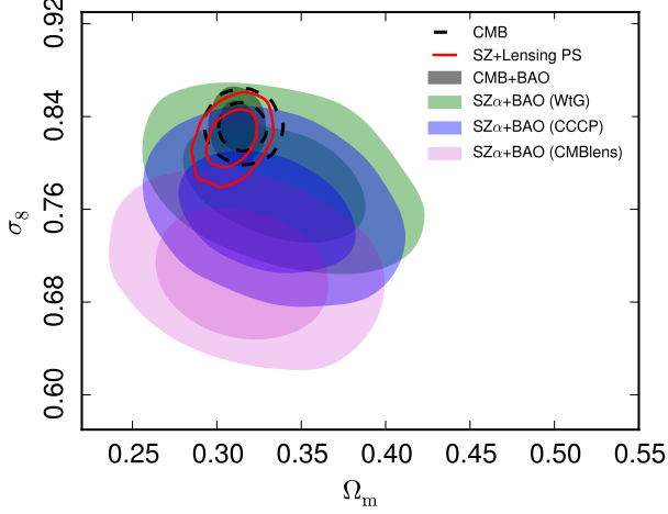
Fig. 7: Comparison of constraints from the CMB to those from the cluster counts in the (\Omega_m, \sigma_8) -plane. The green, blue and violet contours give the cluster constraints (two-dimensional likelihood) at 68 and 95 % for the WtG, CCCP, and CMB lensing mass calibrations, respectively, as listed in Table 2. These constraints are obtained from the MMF3 catalogue with the SZ+BAO+BBN data set and \alpha free (hence the SZ \alpha notation). Constraints from the Planck TT, TE, EE+lowP CMB likelihood (hereafter, Planck primary CMB) are shown as the dashed contours enclosing 68 and 95 % confidence regions (Planck Collaboration XIII 2015), while the grey shaded region also includes BAO. The red contours give results from a joint analysis of the cluster counts and the Planck lensing power spectrum (Planck Collaboration XV 2015), adopting our external priors on n_s and \Omega_b h^2 with the mass bias parameter free and \alpha constrained by the X-ray prior (hence the SZ notation without the subscript \alpha ).
