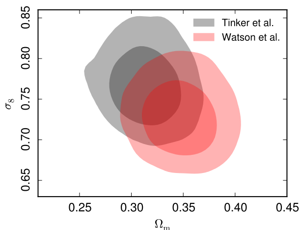
Fig. A.2: Robustness to the choice of mass function. The grey shaded contours give the cosmological constraints when using the Tinker et al. (2008) mass function, corresponding to our final result. This is compared to constraints obtained when using the Watson et al. (2013a) mass function, shown as the red shaded contours. In this figure we adopt the SZ+BAO+BBN data set and the CCCP mass bias prior.
