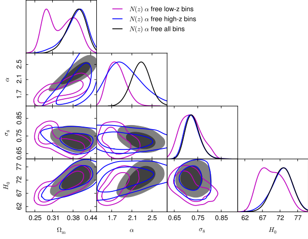
Fig. A.4: Comparison of constraints from the full redshift distribution (in black) to those from the redshift split: two bins at z < 0.2 (in purple) and eight bins at z > 0.2 (in blue). The constraints are obtained with the one-dimensional likelihood when leaving \alpha free, and the black curves and contours reproduce those from Fig. 5.
