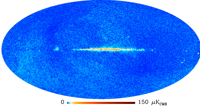
Fig. 19. Difference between the combined weighted polarization maps for Planck and WMAP at 1^\circ resolution, defined as \left[(Q_{\text{Planck}} - Q_{\text{WMAP}})^2 + (U_{\text{Planck}} - U_{\text{WMAP}})^2\right]^{1/2} .
