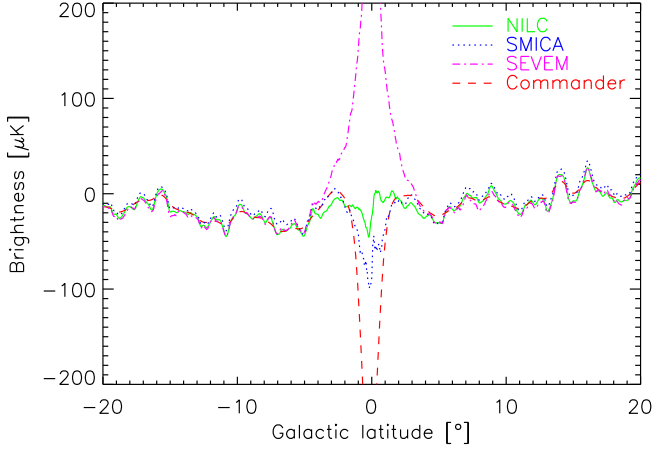
Fig. 26. Mean brightness vs. Galactic latitude, b , in the Planck CMB maps from Planck Collaboration IX (2016) , in the range |l| < 60^\circ . Solid green: NILC; dotted blue: SMICA; dot-dashed magenta: SEVEM (all at 5 arcmin resolution); dashed red: baseline Commander model at 1^\circ resolution ( Planck Collaboration X 2016 ). The first three methods all use inpainting to fill masked regions around bright compact features in some or all of the input maps: pixels affected by this have been omitted from the averaging. High amplitudes close to b = 0 are due to residual foreground contamination.
