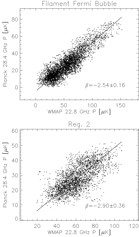
Fig. 31. T - T plots between the polarization amplitude maps of WMAP K-band and Planck 28.4 GHz. The two plots correspond to the regions defined in the left panel of Fig. 30. The Fermi bubble filament shows a flatter spectrum than the control region.
