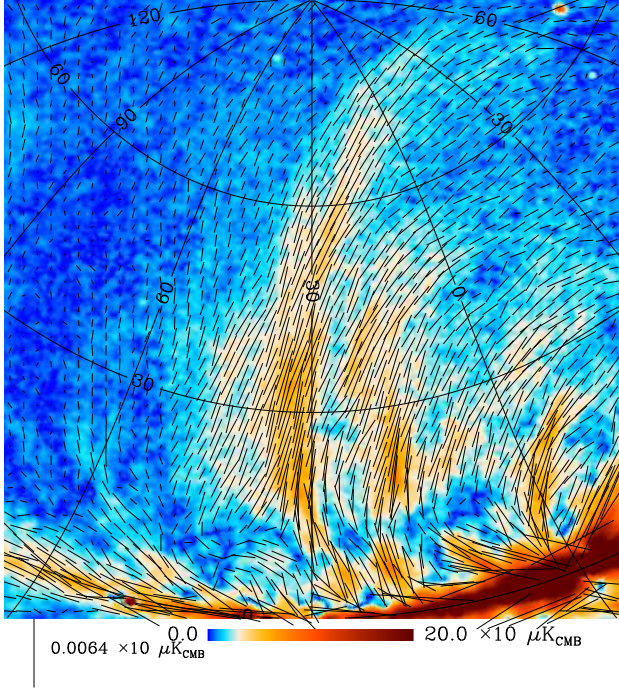
Fig. 25. Combined 28.4 GHz polarization map at 1^\circ resolution of the North Polar spur and the region outside its perimeter, including filament X of Vidal et al. (2015), which leaves the Galactic plane at a shallow angle from near l = 36^\circ , and the l = 45^\circ feature between filament X and the NPS. Colour scale is asinh, but the length scale for polarization line elements remains linear, as in all our figures.
