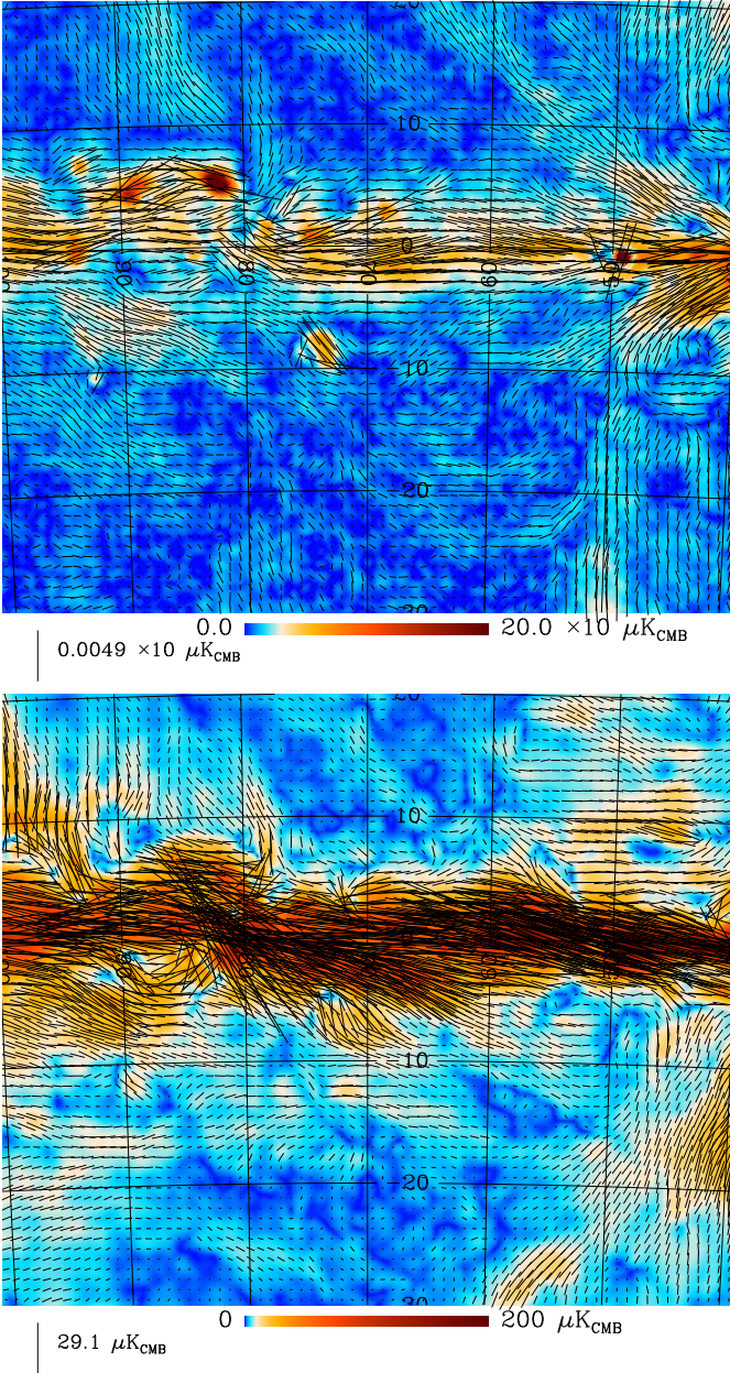
Fig. 29. Top: combined polarization map with magnetic field vectors overlaid, centred on (l, b) = (70^\circ, -7.5^\circ) showing several polarized arches south of the plane. Bright compact features along the plane are all SNRs: DA 530 (G93.3+6.9); HB 21 (G89.2+4.7); W 63 (G82.2+5.3); CTB 87 (G74.9+1.2); the Cygnus Loop (G74.0–8.5); CTB 80 (G69.0+2.7); and W 51C (G49.1–0.6). The large spur at l \approx 50^\circ is the SPS. Bottom: dust polarization in the same region as seen at 353 GHz. Maps are rectangular projections and have an asinh colour scale.
