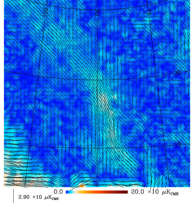
Fig. 27. Combined polarization map of the Cygnus spur, the right-hand end of Loop III. The map is centred at (l, b) = (90^\circ, +27^\circ) and the graticule has a 15^\circ spacing.
