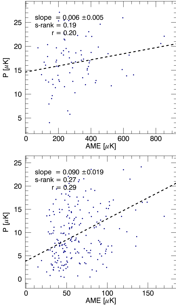
Fig. 34. T – T plots between the polarization and AME intensities (both in units of \mu\text{K} at 22.8 GHz). Top: Perseus; bottom: Pegasus plume. The scatter is mostly due to thermal noise in the polarization map (uncertainties in the polarization intensity in these regions are typically around 5 \mu\text{K} ). The fitted slope gives the polarization fraction for the region, based on the linear fit (dashed line).
