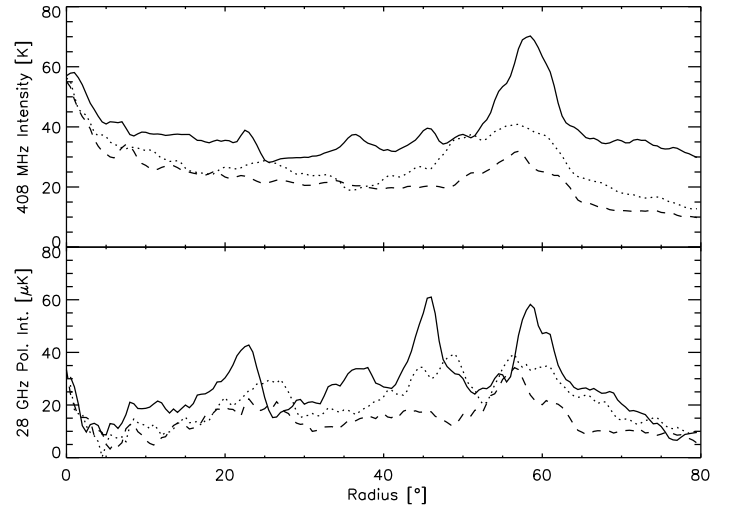
Fig. 23. Profiles of Loop I in total intensity at 408 MHz (Remazeilles et al. 2015) and in our combined Planck-WMAP polarized intensity image at 28.4 GHz. Profiles are along radial cuts beginning at the nominal centre of the loop, (l, b) = (329^\circ, 17.5^\circ) and are averaged over a 10^\circ -wide sector in position angle, at position angles 75^\circ (solid line), 50^\circ (dotted), and 25^\circ (dashed). They cross the North Polar spur at b = 22^\circ, 43^\circ , and 61^\circ , respectively.
