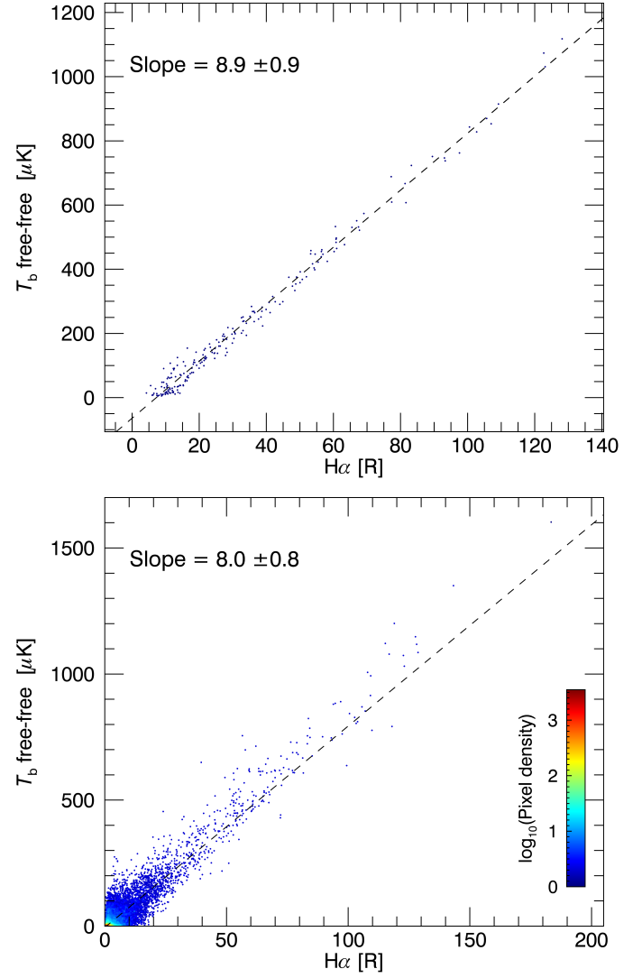
Fig. 4. Top: T - T plot of the free-free amplitude at 22.8 GHz against the H\alpha intensity [R] in the Gum Nebula (see Fig. 5 for the location of the region). Bottom: T - T plot for 85 % of the sky. Regions that show large dust absorption have been masked out, mostly within |b| \lesssim 7^\circ .
