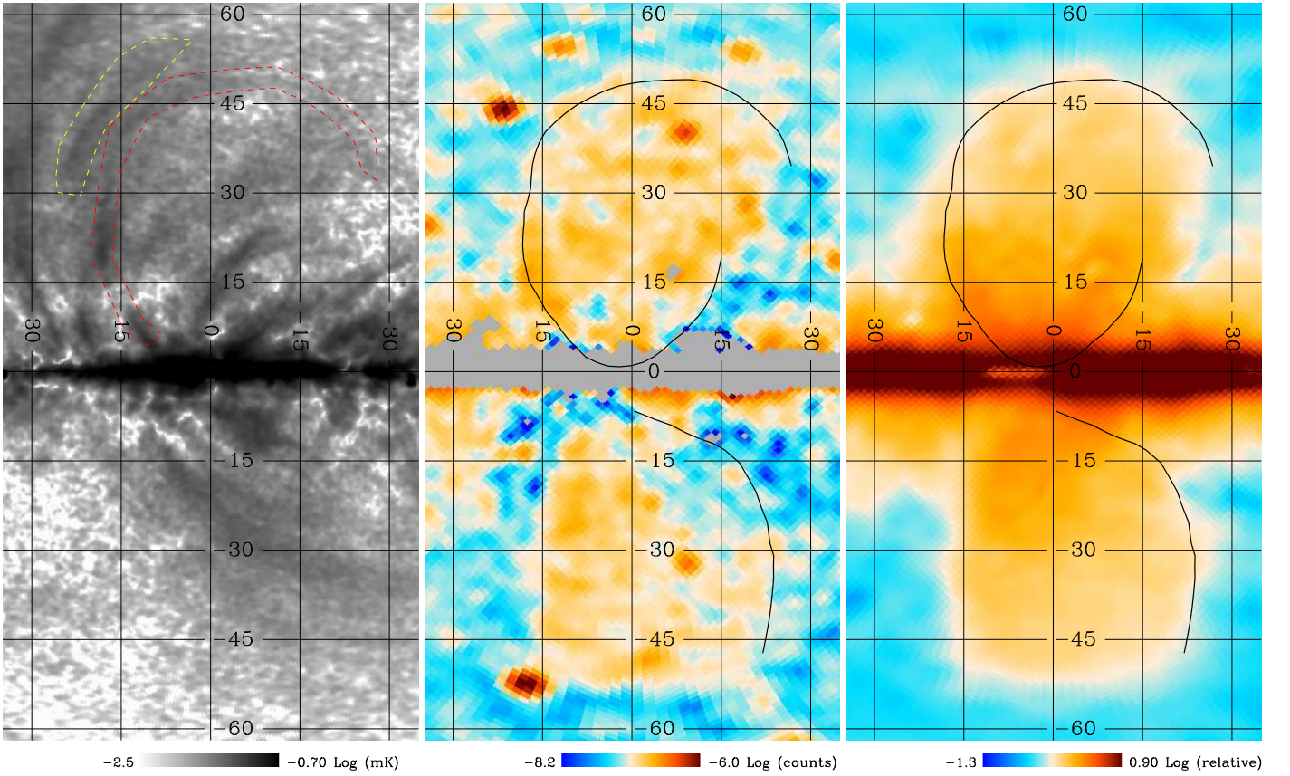
Fig. 30. Left: cartographic projection of the combined Planck -WMAP polarization amplitude, centred at the Galactic centre, with graticule lines at 15° intervals. The regions defined by red and yellow dashed lines were selected to calculate a polarized spectral index; in red is the filament around the Fermi bubble and in yellow a control area. Centre: cartographic projection of the 10–500 GeV map from Ackermann et al. (2014), with the \pi^0 emission subtracted as described in the text, showing the Fermi bubbles. Right: Fermi bubbles component from Selig et al. (2015). The black outline corresponds to the centre of the narrow filaments visible in the polarization map on the left.
