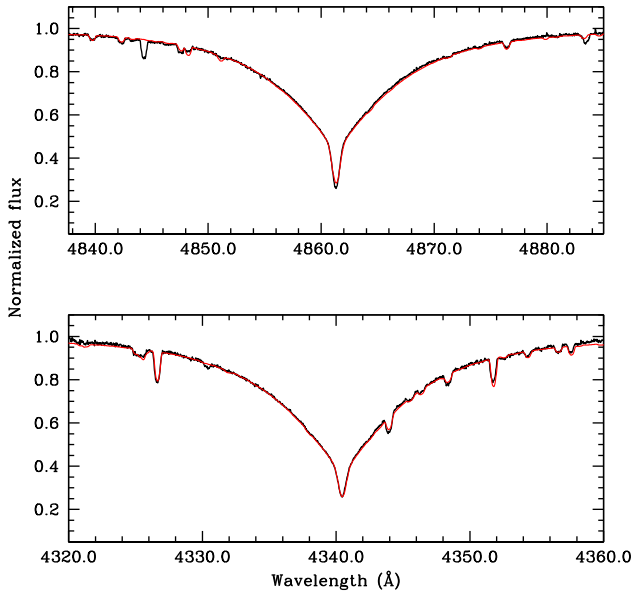
Figure 1. Comparison between observed and computed H \beta and H \gamma profiles, computed by ATLAS12 and SYNTHS as explained in the text.
