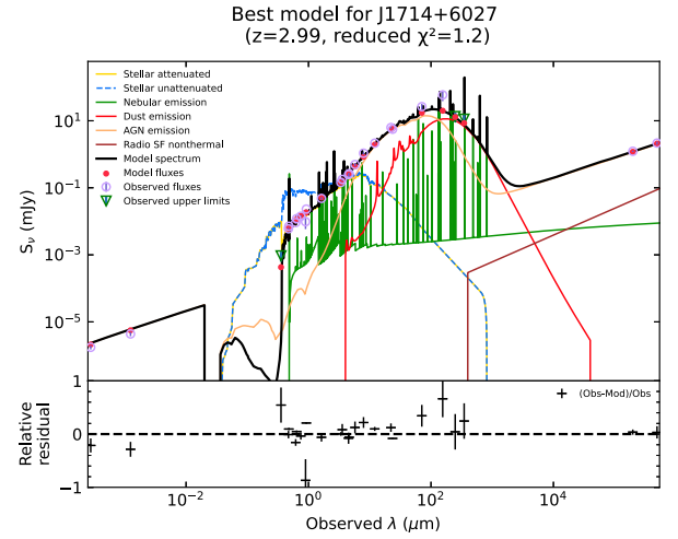
Figure 5. Best-fit SED fitting result from CIGALE and relative residual. The line styles for each module are listed in the key. Relative residual is defined as (\text{Obs}-\text{Mod})/\text{Obs} , where Obs is the observation data and Mod is the model prediction.
