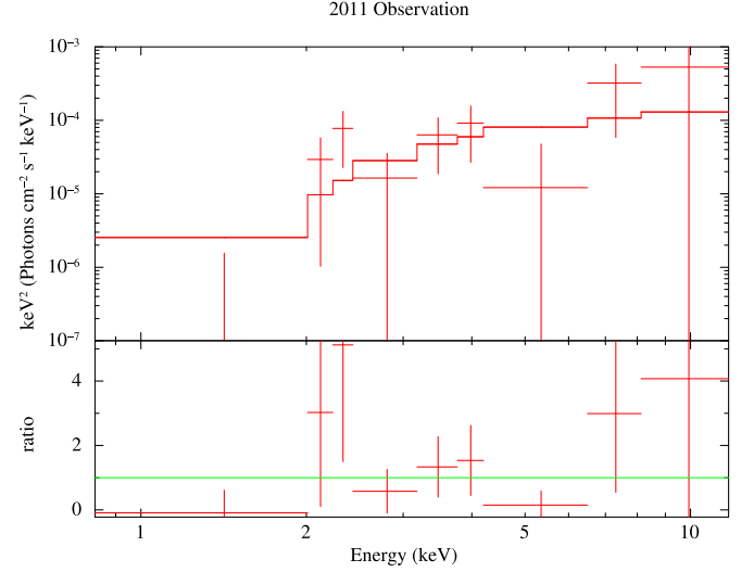
Figure 2. The 2011 XMM-Newton observed X-ray spectrum (in observed frame) of J1714+6027 fitted using the phenomenological model described in Section 2.2.1. The spectra are grouped with a minimum of 2 counts per bin. The red points correspond to the data, and the solid line is the best-fit model prediction.
