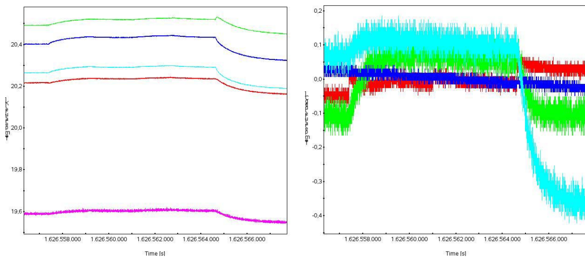
Figure 6 LFI front-end unit (left) and BEU temperature during part 1 On the left panel: green , blue, cyan, red, magenta; on the right panel: green, cyan, red, blue
