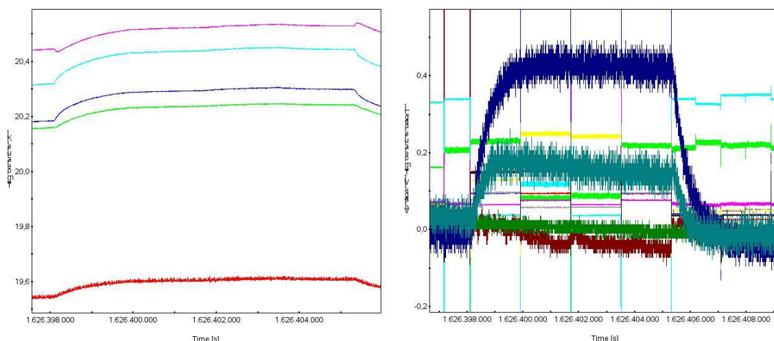
Figure 4 LFI front-end unit (left) and BEU temperature during part 1 On the left panel: green , blue, cyan, red, magenta; on the right panel: green, cyan, red, blue
