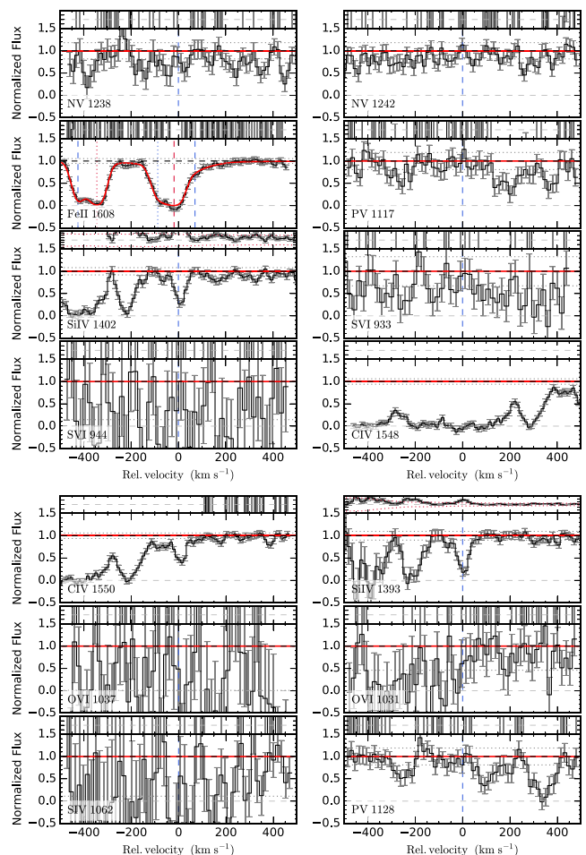
Figure B8. GRB121024A.
