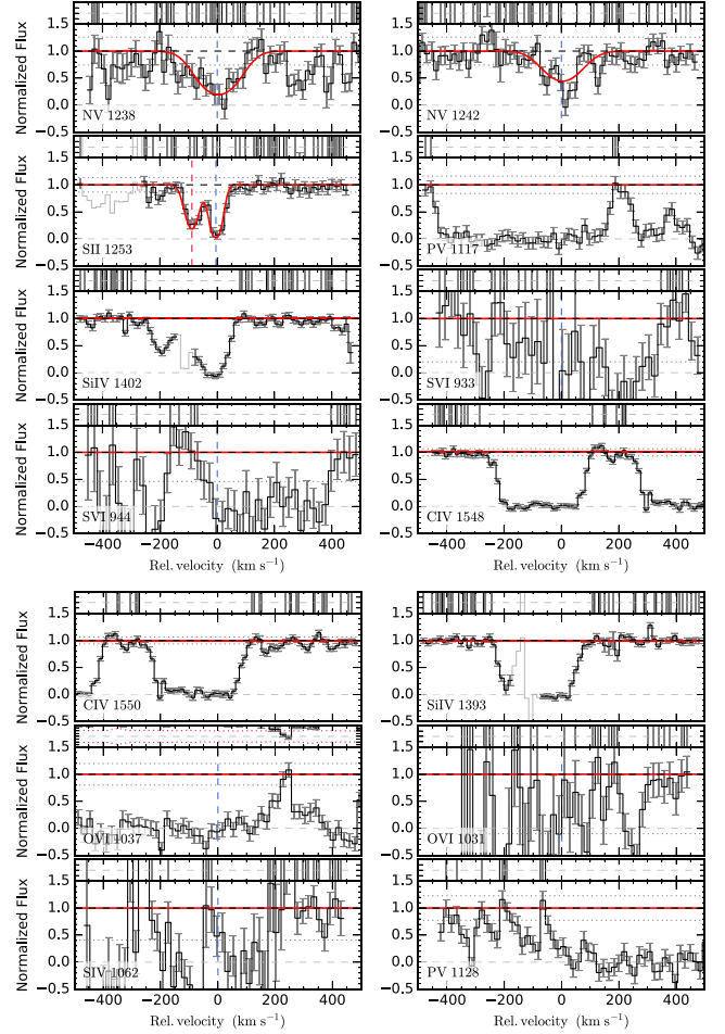
Figure B4. GRB111008A. The spectrum has been binned by a factor of 2.
