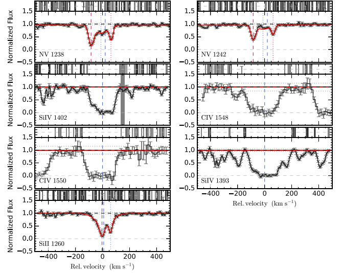
Figure B10. GRB130606A.
