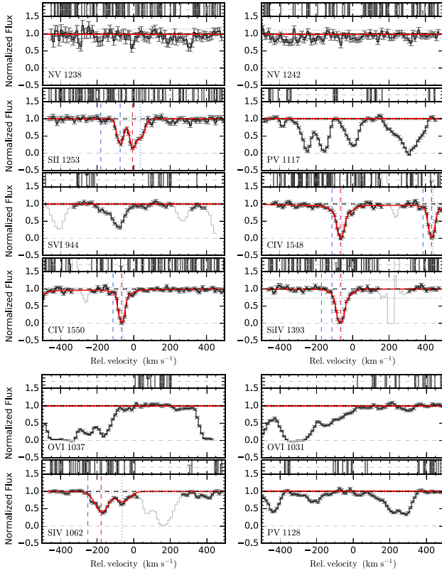
Figure B16. GRB160203A.
