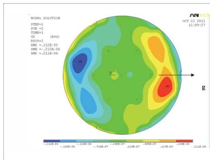
Fig. 6. The deflections of the thin shell [m] in the directions perpendicular to the optical surface. The shell PTV deflection is about 0.42 micron before active compensation.
