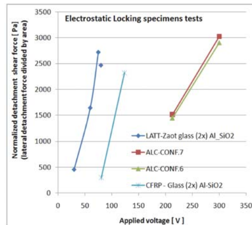
Fig. 3. P_z values at different applied voltage required P_z pressure can be achieved by using a voltage of about 120-150 V (cyan line).
