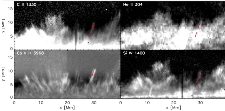
Figure 9. Simultaneous images of spicules in Ca II H 3968 Å (Hinode), C II 1330 Å and Si IV 1400 Å (IRIS) and He II 304 Å (SDO/AIA). Future coordinated observations with DKIST, ALMA and other observatories are key to addressing unresolved questions about spicule heating and their role in the mass and energy balance of the transition region and corona. Image from Skogsrud et al. (2015).
