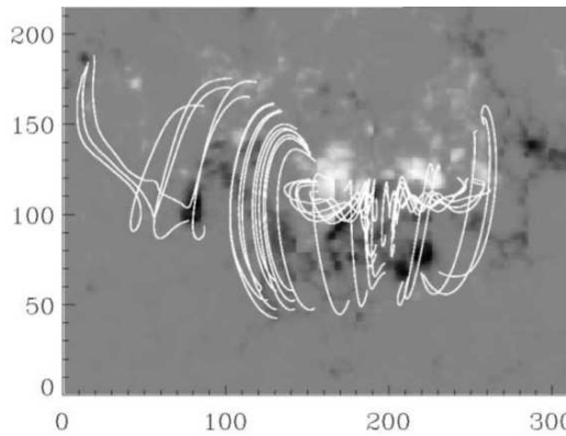
Figure 5. Nonlinear force-free magnetic field reconstruction of NOAA Active Region 9077 before the X5.7/3B (10:24 UT) flare on 14 July 2000, based on vector magnetograms taken at the Huairou Station of the Beijing Astronomical Observatory. The photospheric longitudinal magnetogram is shown in the background for reference. Field lines trace the magnetic flux rope above the neutral line and the overlying arcade field. From Yan et al. (2001).
