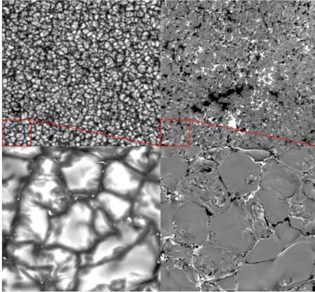
Figure 1. Top: SST CRISP observation of the quiet Sun with 0.15'' resolution ( \sim 100 km), displaying Stokes I and Stokes V. Images courtesy L. Bellot Rubio (IAA-CSIC), S. Esteban Pozuelo (IAA-CSIC) and A. Ortiz (ITA, University of Oslo) http://www.est-east.eu/est/index.php?option=com_content&view=article&id=774&lang=en?quiet-sun-magnetic-fields-2-2-2 . Bottom: quiet Sun simulation with 4-km grid spacing (comparable to DKIST effective resolution of \sim 20 km) displaying bolometric intensity and vertical magnetic field strength (in the range \pm 200 G) at optical depth 0.1. Simulation from Rempel (2014).
