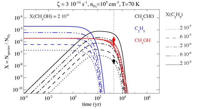
Figure 3. Evolution of acetaldehyde ( \text{CH}_3\text{CHO} , black), ( \text{C}_2\text{H}_5 , blue) and methanol ( \text{CH}_3\text{OH} , red) abundances in the shock as a function of time. Observed abundances (colour circles) are overplotted at the shock age ( t_{\text{shock}} \sim 2000\text{ yr} , vertical dotted line). The evolution is computed from steady-state values in the cloud ( n_{\text{H}_2} = 10^4\text{ cm}^{-3} , T_{\text{kin}} = 10\text{ K} , \zeta = 3 \times 10^{-16}\text{ s}^{-1} ) by enhancing the gas temperature and density ( n_{\text{H}_2} = 10^5\text{ cm}^{-3} , T_{\text{kin}} = 70\text{ K} ), and the abundance of molecules which are thought to be sputtered off dust grain mantles. We set X_{\text{CO}_2} = 6 \times 10^{-5} and X_{\text{OCS}} = 6 \times 10^{-6} as in Podio et al. (2014), X_{\text{CH}_3\text{OH}} = 2 \times 10^{-6} (Mendoza et al. 2014), and vary the abundance of \text{C}_2\text{H}_5 between 2 \times 10^{-7} and 2 \times 10^{-5} .
