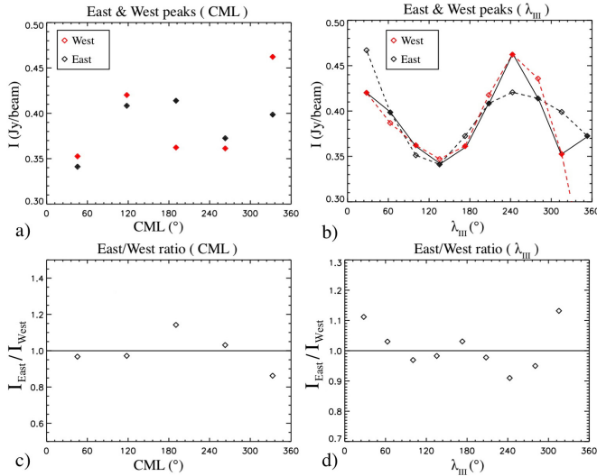
Fig. 12. a) East and west peak intensities in each frequency-averaged image as a function of the CML at the middle of the 2-h interval corresponding to each image. b) East and west peak intensities – as a proxy of the peak emissivity – as a function of \lambda_{III} , derived from a) following the sketch of Fig. 11. Measured values are filled diamonds connected by the solid line. Open diamonds are interpolated from a spline adjustment of east and west measurements separately. Dashed lines are the two resulting independent determinations of the peak emissivity profiles versus \lambda_{III} . c), d) east-to-west peak intensity ratios deduced from panels a) and b) .
