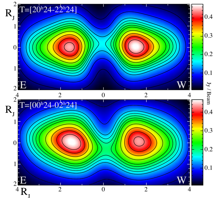
Fig. 9. Simulated synchrotron images derived from Salammbô-3D (see text) of the emission averaged over the full band at two periods: i) [20h24–22h24] UT (CML = [9^\circ\text{--}82^\circ] ), min/max = [8 \times 10^{-3}, 0.475] Jy/beam and ii) [00h24–02h24] UT (CML = [154^\circ\text{--}227^\circ] ), min/max = [8 \times 10^{-3}, 0.467] Jy/beam. The synchrotron maps were computed with the same observation parameters as in Figs. 5b and d. Contours highlight the brightness by steps of 10% of the maximum.
