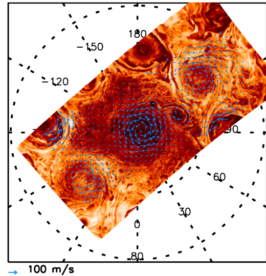
Figure 4: Wind velocity amplitudes (panel a) and directions (panel b) over the north pole, derived for the N1 case of Table 2, as corrected to achieve maximum azimuthal symmetry of wind speed around the centre of NPC. Figure A1 provides analogous information for cases N2, N3 and N4.
