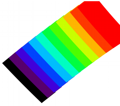
Figure A3: actual scheme of individual JIRAM images used to build the background image of figures 2b and 3b. Each colour corresponds to a different image inside the sequence 170202_114231. Acquisition times of images were spaced in intervals of 30 seconds.
