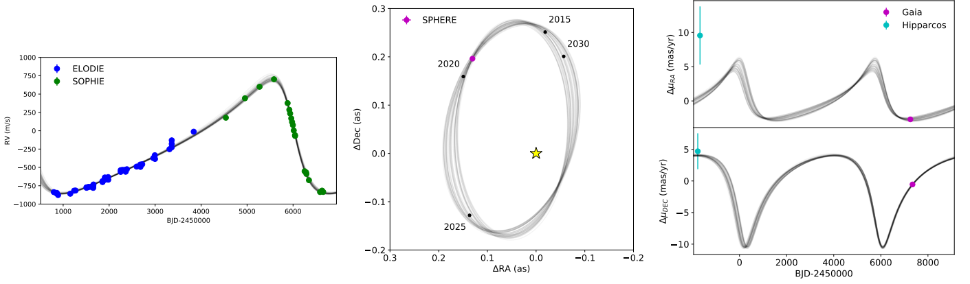
Fig. 2. Sample of 50 model orbits fitted on the HD 72946B data (colored points) from RV ( left ), imaging ( middle ), and astrometry ( right ). In the middle panel, the yellow star marks the location of the primary star, and the black dots show the median predicted position for given epochs.
