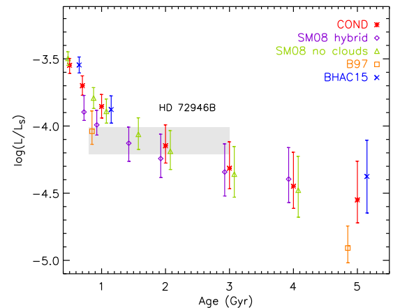
Fig. 5. Bolometric luminosity vs. age of HD 72946B (gray area) compared to evolutionary tracks from the models COND (Baraffe et al. 2003), Saumon & Marley (2008) (for two treatments of the clouds), Burrows et al. (1997), and Baraffe et al. (2015) assuming the mass range for the companion from the orbital fit (data points). Small horizontal offsets are applied to all models except for COND for clarity.
