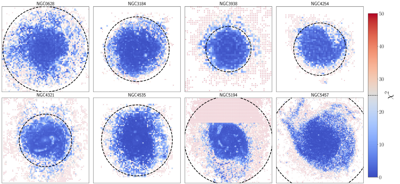
Figure 2. Final \chi^2 maps for the full sample of galaxies for cells of 8 arcsec. The blue coloured squares are the accepted values (below the threshold of 25, highlighted with a dotted line in the colourbar), and the red shaded points are the discarded ones lying over the threshold. For NGC 5194, each point with \delta > 47.24052 has been discarded in order to remove contamination from the M51b companion (they form a second tight sequence below the accepted cells). The dotted circle is the galaxy r_{25} reported in Table 1. Almost every cell in the innermost galaxy regions is accepted. In the outer part of the disc, the spiral arms tend to produce acceptable fits with respect to the non-spiral part of the galaxies, as it is clear from NGC 5457.
