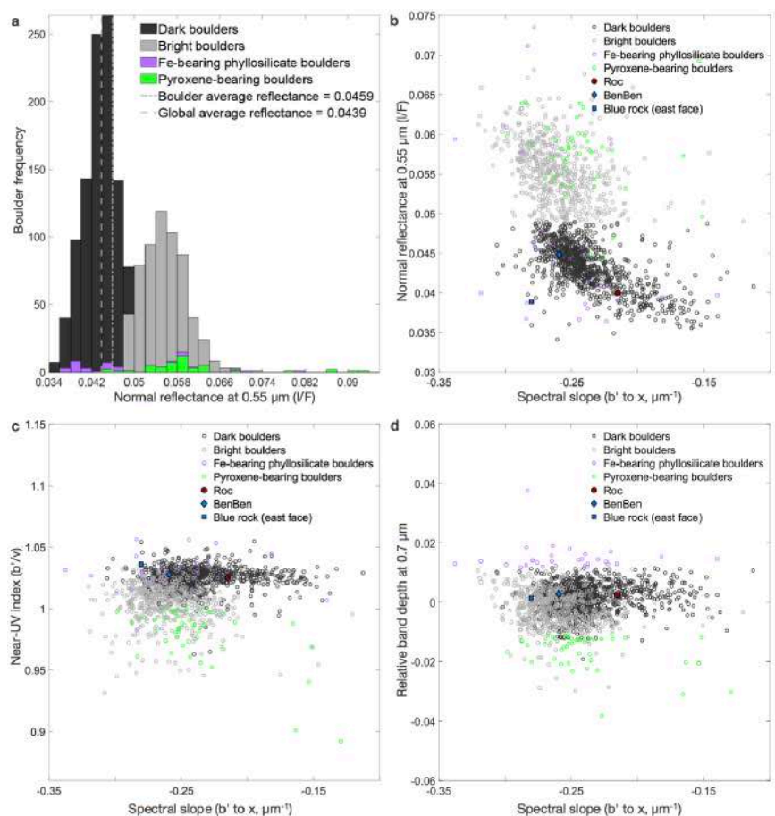
Fig. 2. Variation of boulder color and reflectance on Benu. (A) Reflectance distribution of boulders ( >5 m) on Benu. The distribution is multi-modal with more than one Gaussian component (31). Shading and colors indicate different classifications of boulders, as indicated in the legend. (B) Normal reflectance versus absolute spectral slope of the same boulder populations; some individual boulders are indicated in the legend. Dark boulders tend to be redder, and their reflectance monotonically decreases with increasing (redder) spectral slopes, whereas bright boulders are bluer and more scattered (31). (C) The near-UV index ( b'/v band ratio) versus the b' to x spectral slope. Dark boulders tend to have a steeper near-UV slope relative to the global average ( >1 ), whereas bright boulders are more often spectrally flat or show a downturn in the near-UV (from the b' to v bands). (D) The relative band depth at 0.7 \mu\text{m} ( w band) versus the b' to x spectral slope. Some boulders show an absorption feature at 0.7 \mu\text{m} (relative w band depth >0 ), indicative of Fe-bearing phyllosilicates. The boulders named Roc (23.6°S, 25.3°E; Fig. 3C) and
