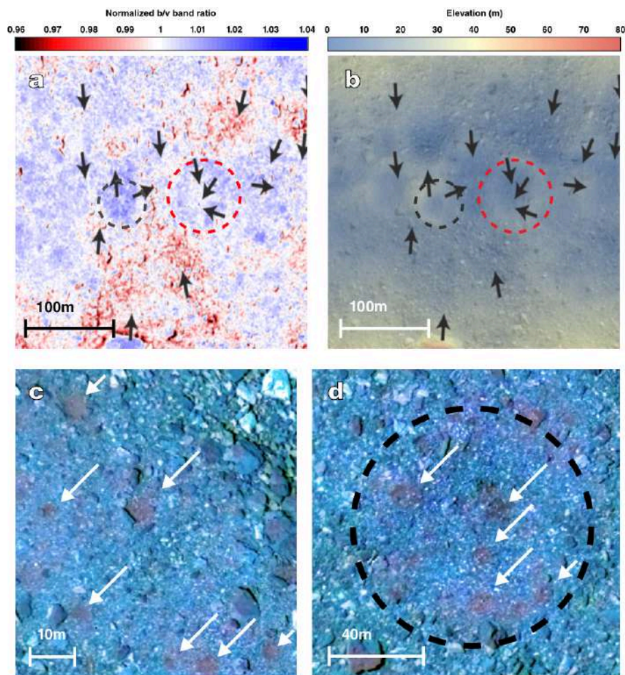
Fig. 4. Examples of crater color. (A) The b/v band ratio map of equatorial craters at 3.05^{\circ}\text{S} , 128.79^{\circ}\text{E} (black dashed line) and 1.06^{\circ}\text{S} , 152.75^{\circ}\text{E} (red dashed line), which have a higher near-UV index and are considered blue units. (B) An elevation map of the same equatorial craters in (A). These blue units correspond with areas that show recent indications of mass movement away from regionally high elevations, such as from crater rims. Black arrows correspond locations of previously mapped mass movement (43). (C and D) RGB color composites images of small craters (indicated by white arrows), shown on the same color scale as Fig. 1A. As indicated by their color, these craters are consistently redder than Bennu's average terrain, with positive to slightly blue b' to x spectral slopes. The blue crater indicated by the dashed black line in (A), (B), and (D) has been overprinted by several smaller reddish craters.
