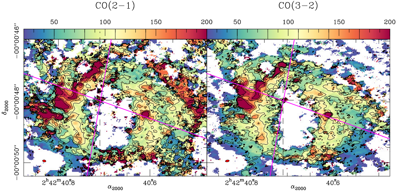
Fig. 9. Velocity-width maps in units of FWHM derived for the CO(2–1) ( left panel ) and CO(3–2) ( right panel ) lines in the CND of NGC 1068, as obtained from the MSR data set. Contours and color scale span the range [20, 200] km s ^{-1} in steps of 30 km s ^{-1} . Symbols and markers as in Figs. 3 and 4.
