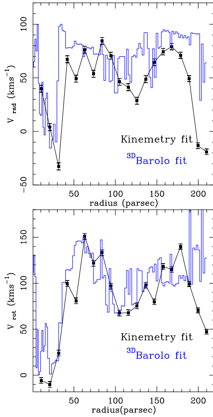
Fig. A.1. Radial profiles of v_{\text{rad}} (upper panel) and v_{\text{rot}} (lower panel) found by 3D Barolo (blue histograms) and kinemetry (black line and markers) to fit the CO(2–1) data of the CNB region out to r \approx 210 pc.
