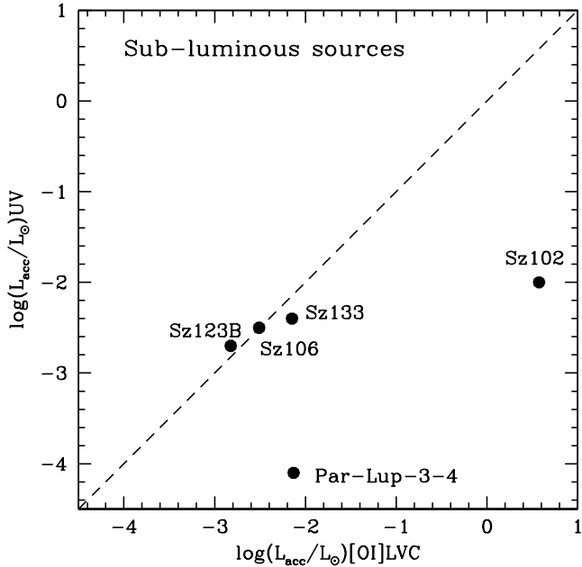
Fig. 8. Accretion luminosity derived by modelling the UV excess is compared with that estimated through the L_{\text{[OI]LVC}} vs. L_{\text{acc}} relationships for the sub-luminous sources.
