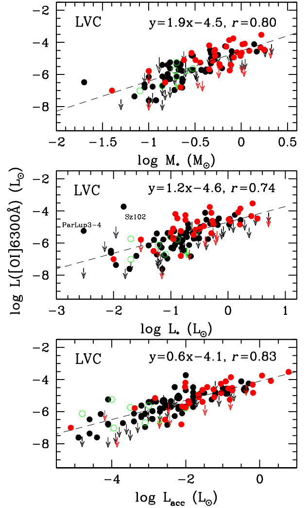
Fig. 4. [O I] 6300 Å line luminosity of the LVC is plotted as a function of, from top to bottom, stellar mass, stellar luminosity and accretion luminosity. Colour codes for the symbols are as in Fig. 3. Arrows refer to 3\sigma upper limits. The dashed line indicates the linear regression whose parameters are given in the upper right corner of each figure, together with the correlation parameter.
