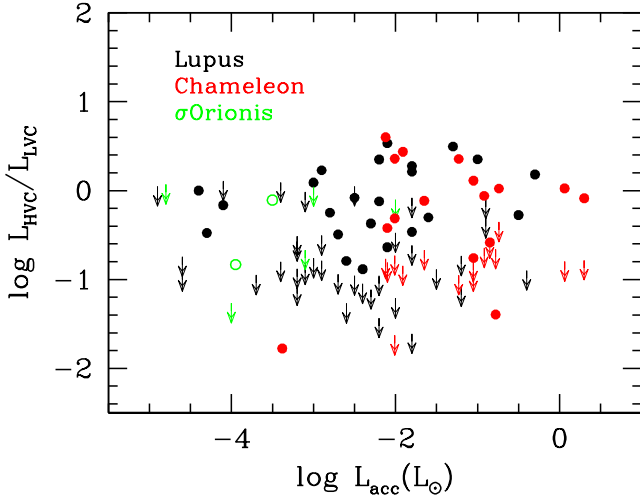
Fig. 3. Ratio between the HVC and LVC [O I] 6300 Å line luminosities as a function of the accretion luminosity. Black, red and green symbols indicate sources in Lupus, Chamaeleon and \sigma Orionis clouds, respectively. Arrows refer to 3\sigma upper limits for the HVC luminosity.
