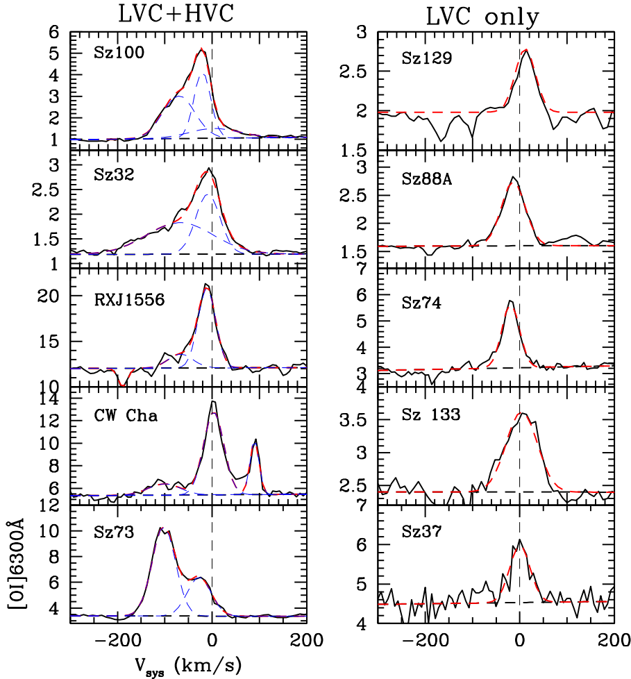
Fig. 1. Examples of [O I] 6300 Å spectra of sources with and without a HVC. Blue-dashed lines indicate the Gaussian profiles used to fit the different components, and the red-dashed line is the final best fit.
