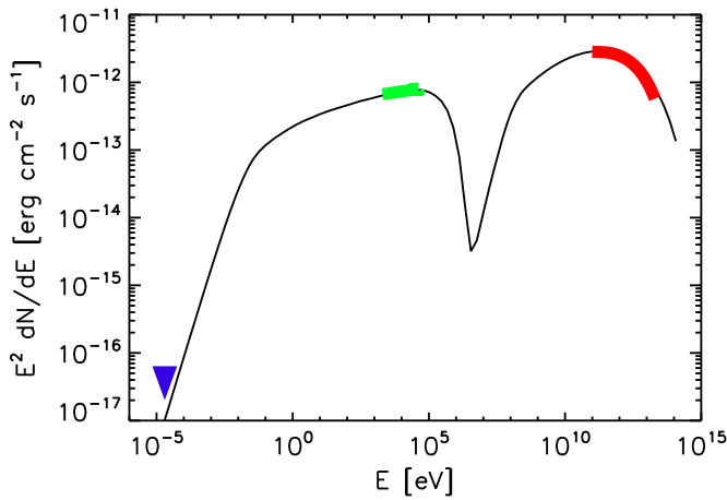
Figure 12. One-zone PWN model fit to the broad-band SED data including the 6 cm radio flux upper limit (blue arrow), G359.95–0.04 X-ray spectrum (green) and 0.1–10 TeV HESS spectrum of HESS J1745–290 (red).
