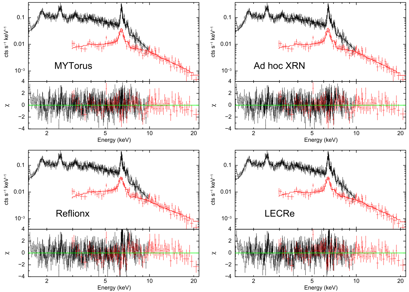
Figure 10. 1.5–20 keV XMM-Newton (black) and NuSTAR (red) spectra of the Bridge fit with the MYTorus (upper left), ad hoc XRN (upper right), reflionx (lower left), and LECRe electron model (lower right).
