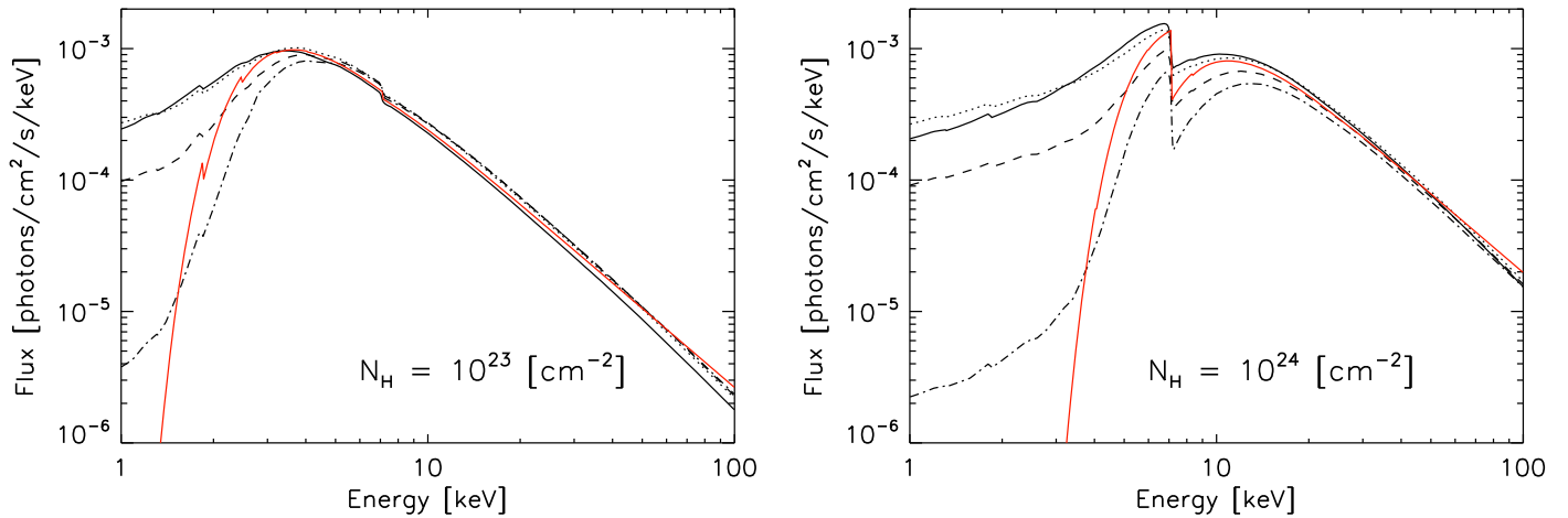
Figure 16. MYTorus model spectra at \theta_{\text{obs}} = 0^\circ (solid), 60^\circ (dotted), 75^\circ (dashed) and 90^\circ (dot-dashed) for the equatorial column density N_{\text{H}} = 10^{23} (left) and 10^{24} \text{cm}^{-2} (right). In all cases, we assumed an input power-law spectrum with \Gamma = 2 . We used the same flux normalization for all the MYTorus model spectra. Note that the model spectra show strong angular dependence at \theta_{\text{obs}} > 60^\circ below \sim 3 keV ( N_{\text{H}} = 10^{23} \text{cm}^{-2} ) and \sim 10 keV ( N_{\text{H}} = 10^{24} \text{cm}^{-2} ). For comparison, we plot an absorbed power-law model (tbabs*powerlaw, red solid lines) with the mean column density of (\pi/4)N_{\text{H}} over all lines-of-sight through the torus (Murphy & Yaqoob 2009), power-law index of \Gamma = 2 and flux normalization roughly adjusted to the MYTorus model spectra in high energy band.
