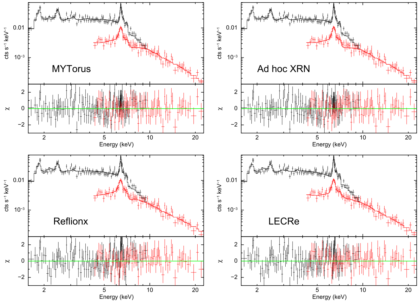
Figure 9. 1.5–20 keV XMM-Newton (black) and NuSTAR (red) spectra of MC1 fit with the MYTorus (upper left), ad hoc XRN (upper right), reflionx (lower left), and LECRe electron model (lower right).
