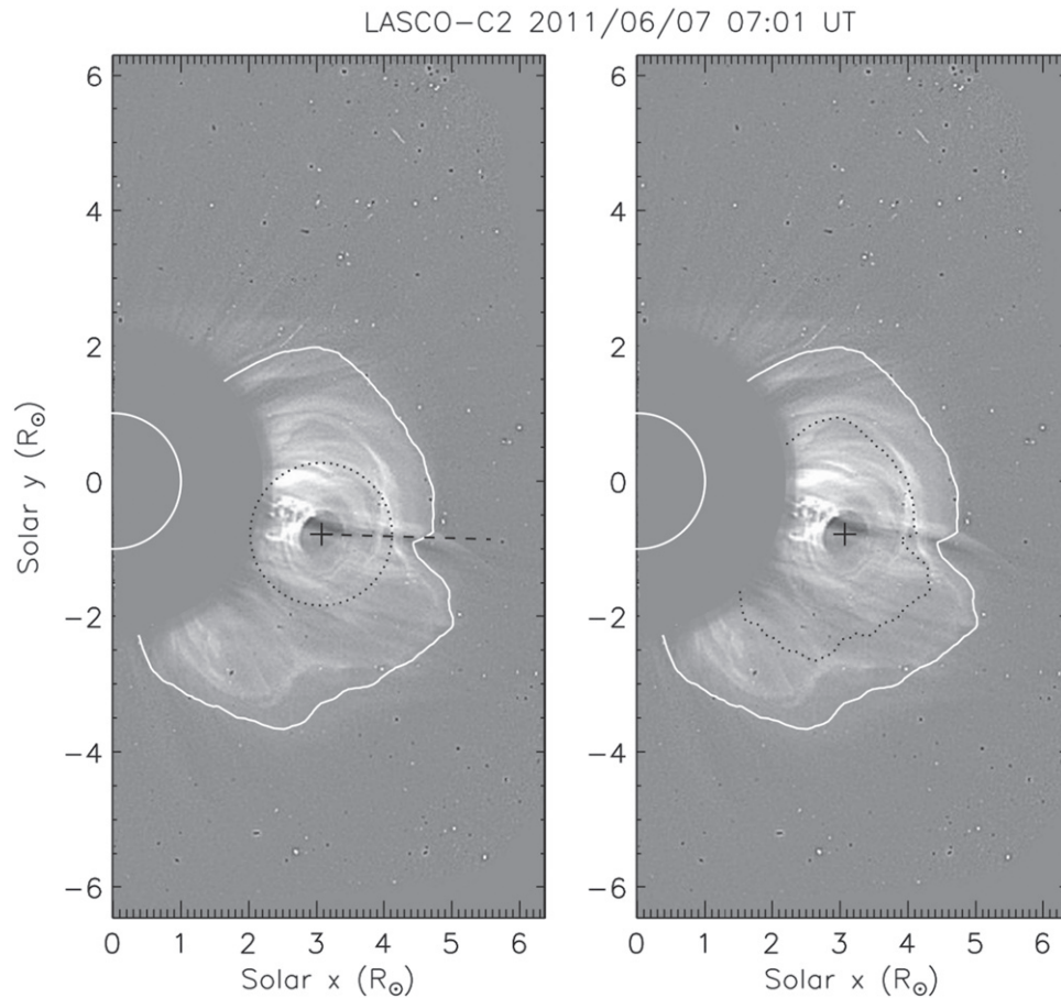
Figure 13. Left: LASCO C2 base-difference image acquired on 2011 June 7 at 07:01 UT and with the contrast of faint features enhanced using the filter provided by the JHelioviewer software. The overplot shows the location of the shock (solid white line), the center of the CME flux rope (plus symbol), and the CME propagation direction (dashed black line). Right: same frame as shown in the left panel, where the overplot provides again the location of the shock (solid white line), the center of the CME flux rope (plus symbol), and the location of the shock driver (black dotted line) as derived by assuming that the relationship between the Mach number at the shock nose and the \Delta/R ratio holds also at different latitudes away from the shock nose (see text).
