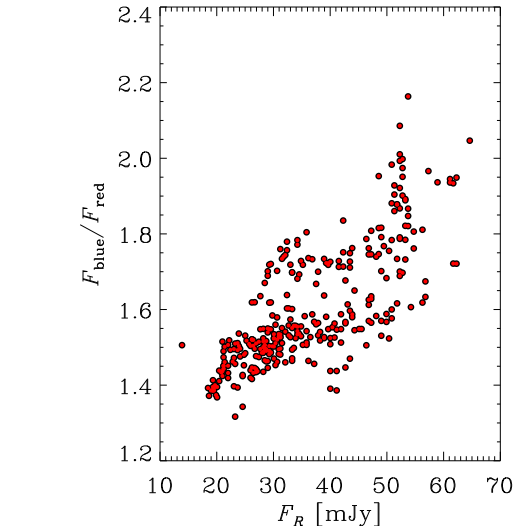
Figure 21. The Mrk 421 optical colour ('blue' to 'red' flux ratio) as a function of the source brightness (observed R -band flux density in mJy).
