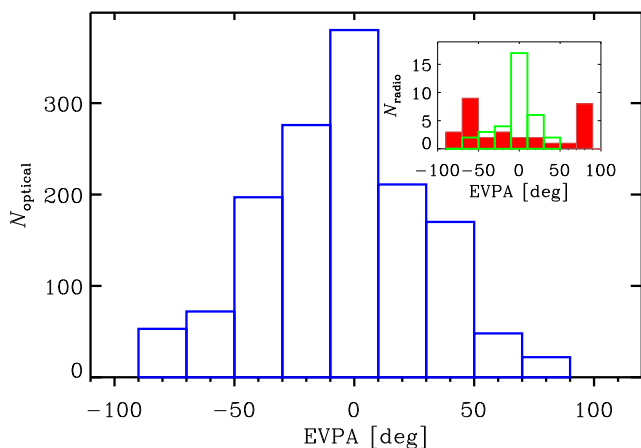
Figure 16. The distribution of the optical EVPA; the inset displays those of the radio EVPA at 43 GHz (green line) and at 15 GHz (red histogram).
