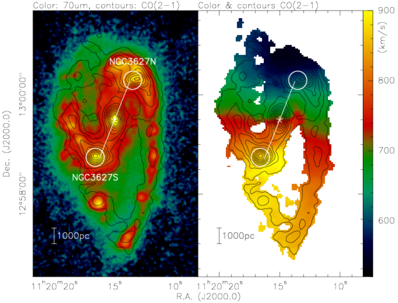
Fig. 1. Herschel 70 \mu\text{m} (Kennicutt et al. 2011) and HERACLES CO(2–1) data of NGC3627 (Leroy et al. 2009). The left panel presents in color the 70 \mu\text{m} emission (logarithmic stretch from 0.0001 to 0.1 Jy pixel ^{-1} ) while the contours show the integrated CO(2–1) emission from 5 to 55 K km s ^{-1} in 5 K km s ^{-1} steps. In the right panel, the color-scale presents the 1st moment map (intensity-weighted velocities), the contours again show the integrated CO(2–1) emission. Circles mark the locations and areas of the PdBI(2–1) primary beams for NGC3627N and NGC3627S. The central star and white line indicate the bar location following Casasola et al. (2011). A linear scale-bar assuming 11.1 Mpc distance is shown in the bottom-left corner.
