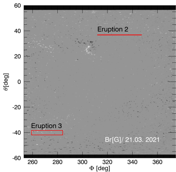
Figure 12 The Br component of the magnetic field from SDO/HMI, for a selected region of the full disk on the 21 March 2021. The red marks represent the position of the prominence 2 and prominence 3 as given in Table 2. X-axis is longitude and Y-axis is latitude in Carrington coordinates.
