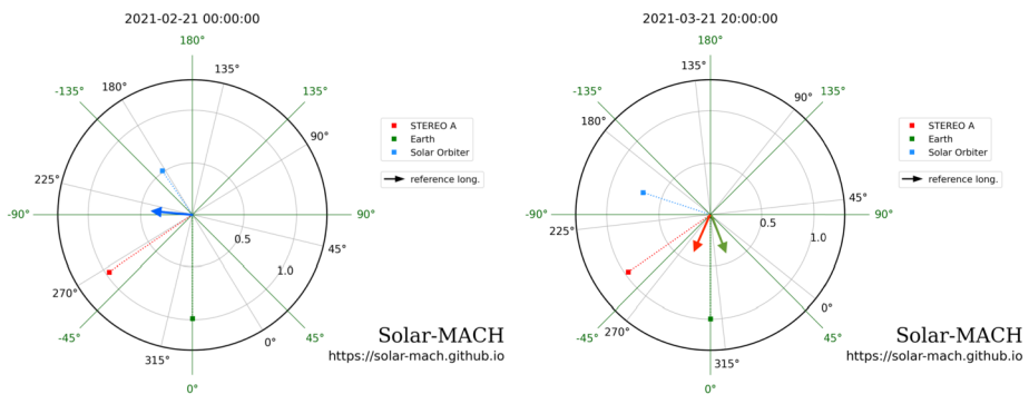
Figure 2 Positions of observing spacecraft on February 21 ( left panel ) and March 21 ( right panel ), 2021 in Carrington (black) and Stonyhurst (green) coordinate systems. The three arrows represent the propagation direction of the three eruptions (blue, green, and red arrows for Eruption 1 , Eruption 2 , and Eruption 3 , respectively) as derived from the GCS reconstruction. The images were created using Solar-MACH ( solar-mach.github.io/ ).
