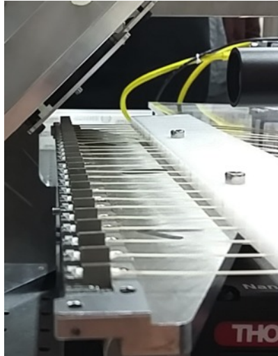
Figure 6: (left) The 24 fibres of the prototype bundle in place on the test setup for automatic measurements. (above) Closeup of the lensed top surface of one of the prisms showing the excellent centration achieved.
