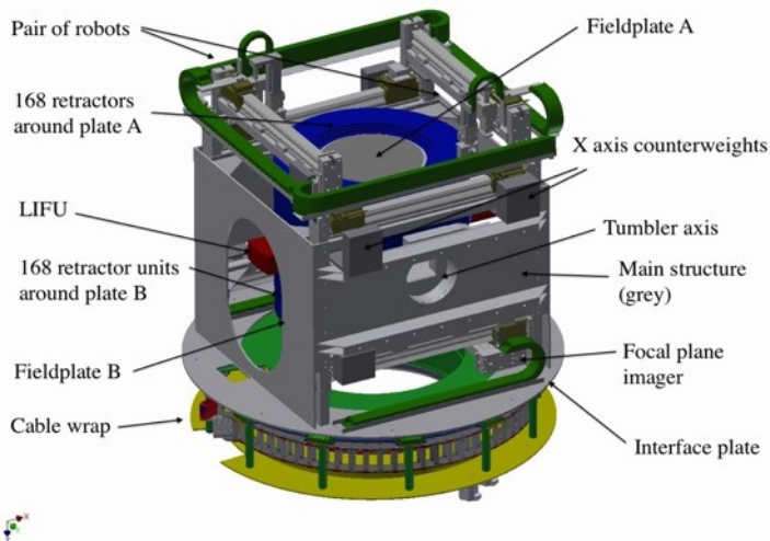
Figure 5: (left) The general layout of the fibre positioner system. (right) Close-up of the two robots in action, showing the \theta axes, gripper units and one of the plate/fibre viewing cameras.
