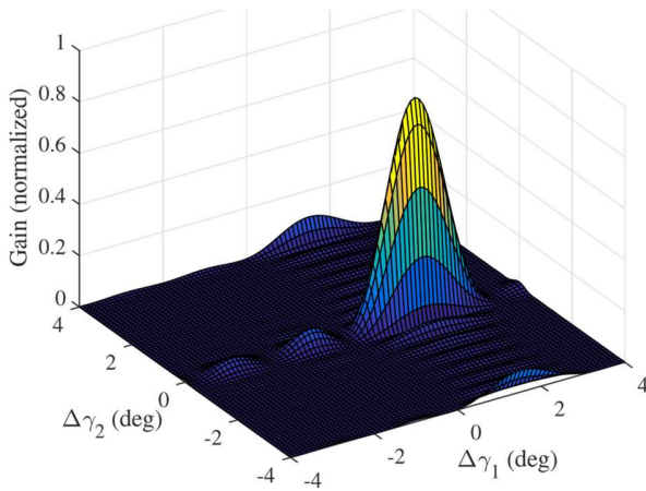
Figure 8: Gain pattern for beam 24: one main lobe, and other minor side lobes.
