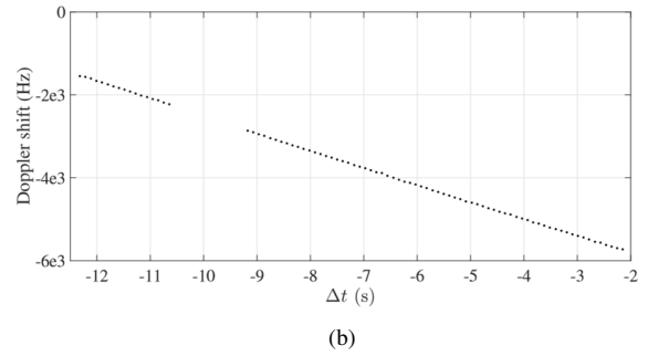
Figure 16: SNR (a) and Doppler shift (b) measurement profiles obtained during Tiangong-1 passage on March 31, 2018 as a function of time delay \Delta t (s) with respect to the TLE-predicted passage epoch.
