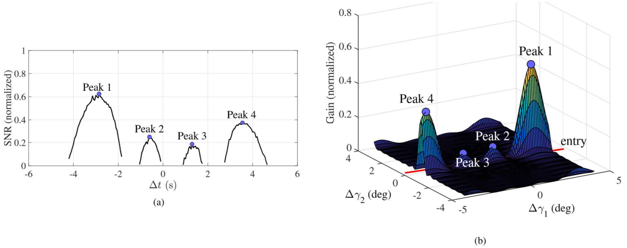
Figure 11: All beams signal peaks association phase for beam 30: (a) SNR profile and signal peaks as a function of the time delay with respect to the expected meridian passage \Delta t , (b) gain pattern profile and associated gain lobes.
