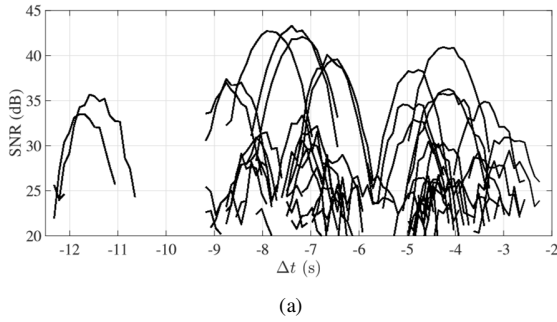
Figure 16: SNR (a) and Doppler shift (b) measurement profiles obtained during Tiangong-1 passage on March 31, 2018 as a function of time delay \Delta t (s) with respect to the TLE-predicted passage epoch.
