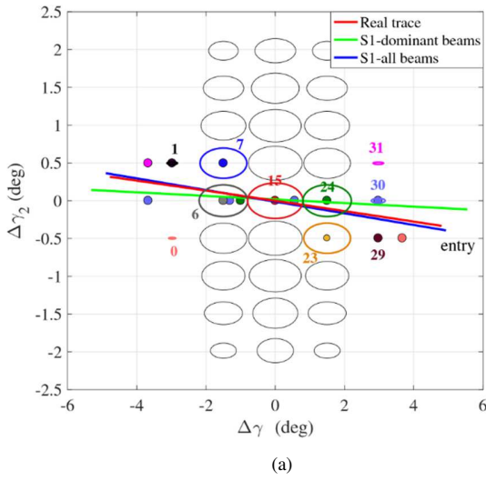
Figure 12: Trace definition for object NORAD ID 417654, passage on April 20, 2018: (a) step S1, trace definition based on SNR peaks, (b) step S2, nonlinear least-squares on the whole SNR profiles.
