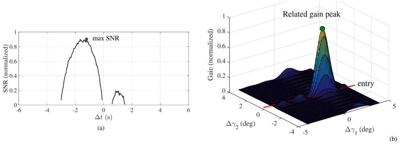
Figure 10: Dominant beams signal peaks association phase for beam 24: (a) SNR profile and signal peak as a function of the time delay with respect to the expected meridian passage \Delta t , (b) gain pattern profile and associated gain lobe.
