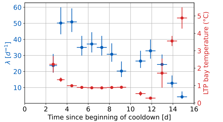
FIG. 6. Glitch occurrence rate \lambda (left scale), and LTP bay temperature (right scale), during CR, as a function of time since the beginning of cooldown. Small temperature changes before day 12 were the result of adjustments of heaters settings aimed at stabilizing the system behaviour. Re-heating to ordinary conditions started at day 12.
