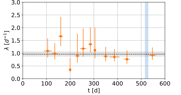
FIG. 5. Glitch occurrence rate \lambda , during OR, vs time t from launch, throughout the entire mission. Points are calculated by grouping glitches observed during runs the start times of which differ by less than a month. Vertical error bars are Bayesian estimates assuming exponential distribution, and corresponds to 68.3% ( 1\sigma ) likelihood (see App. B). Horizontal error bars correspond to the total duration of the considered epoch. The dashed line, and the associated gray shaded area, represent, respectively, the mean rate and its error from the Bayesian estimate. The blue shaded area indicates the epoch of CR.
