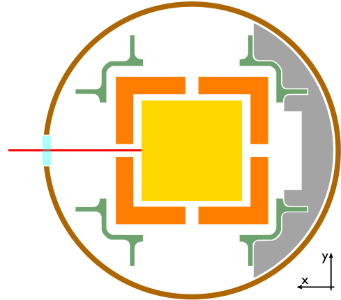
FIG. 15. Schematic representation of the GRS, horizontal section. The yellow square is the Au-Pt TM. The orange hollow square represents the EH, whose mid section carries four symmetric holes, one of which is the input port for the laser beam (in red). The green part is the section of a titanium structure that holds the various elements together, while in gray is the specially shaped tungsten gravitational balance mass. The brown circle is the section of the vacuum chamber, while the cyan rectangle represent the optical window to transmit the laser beam.
