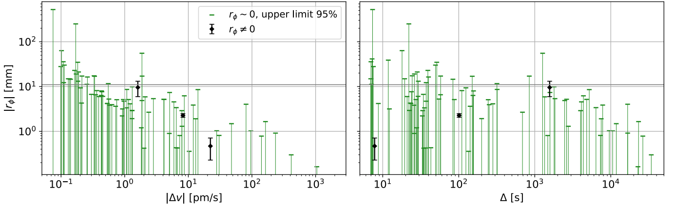
FIG. 14. Absolute lever arm |r_\phi| , as defined in Eq. (10), as a function of absolute impulse |\Delta v| (left) and duration \Delta (right), for impulse-carrying glitches of OR. The black data points represent the glitches for which the lever arm has been found to be significantly different from zero. The green horizontal segments represent the upper bound for |r_\phi| for glitches for which |\Delta\Omega_\phi| \leq \delta\Omega_\phi . For 9 of the 98 impulse-carrying glitches of the OR, we were not able to perform the analysis on the \Delta\gamma_\phi(t) data series. The gray horizontal line refers to the 11 mm “electrical” reference, as described in text.
