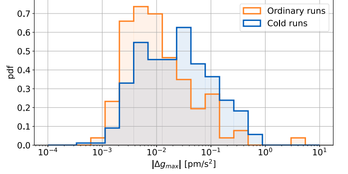
FIG. 10. Histogram of peak amplitude |\Delta g_{\text{max}}| for all glitches of Fig. 7. The probability density is for the logarithm of the amplitude.
