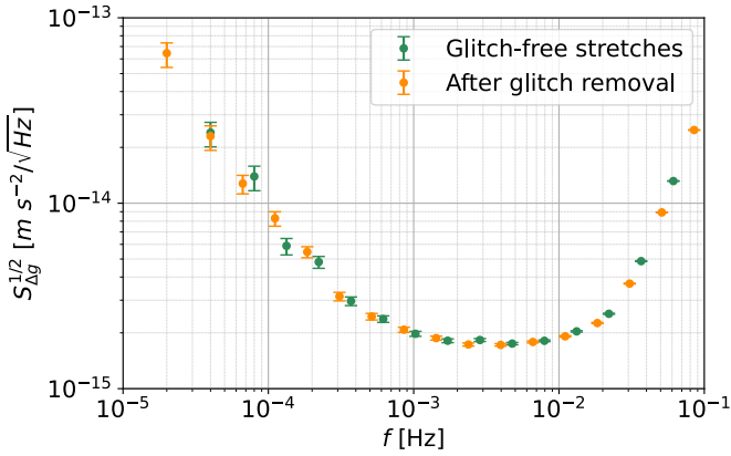
FIG. 3. Amplitude spectral density (ASD) S_{\Delta g}^{1/2}(f) of quasi-stationary noise, vs the frequency f , of the best noise run of February 2017. Green data points: ASD of glitch-free stretches only. Orange data points: ASD of residuals after glitch removal. Errors represent 68% confidence intervals.
