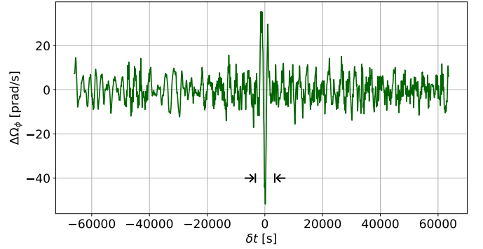
FIG. 13. An example of the \Delta \Omega_\phi(\delta t) series for one of the very few glitches with significant associated torque. The value in \delta t = 0 is the result of the fit for native data. The arrows indicate the interval excluded for the sake of error evaluation.
