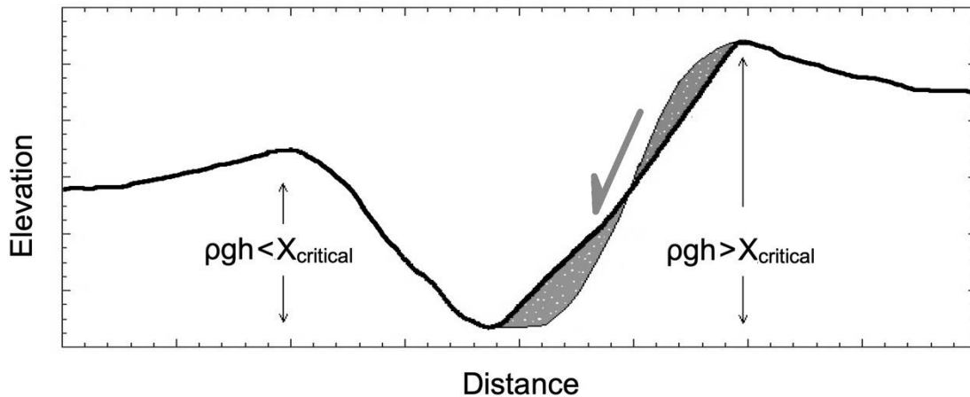
Figure 25. Schematic illustration of principle of asymmetric overburden rim failure in simple craters on slopes. X_{\text{critical}} is proportional to the failure criterion for impact disrupted crustal material. At smaller diameters X_{\text{critical}} is not exceeded (or is at larger diameters) anywhere in the crater.
