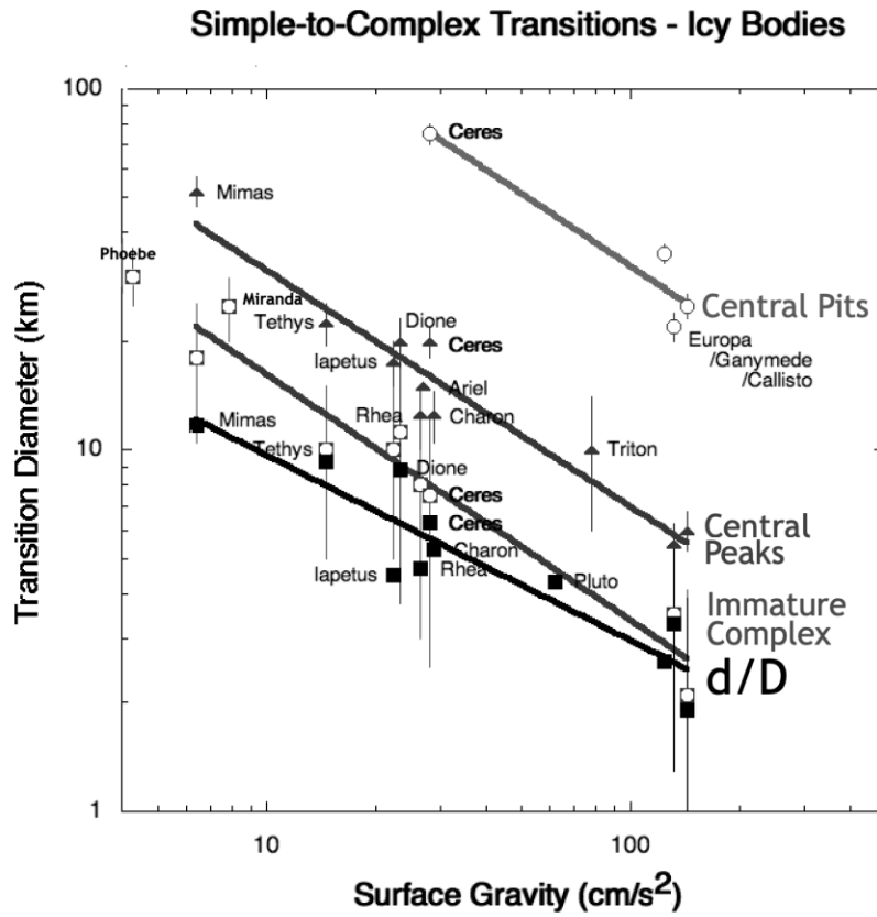
Figure 27. Transition diameters for crater types and depth/diameter inflection on Ceres and icy satellites. Lines are best fits through data.
