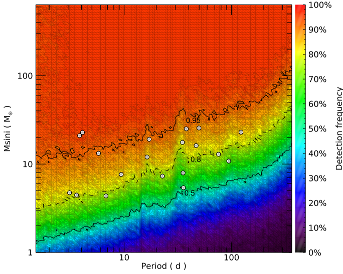
Fig. 23. Colour-coded HARPS precision detection frequency map for the whole 20-systems sample studied in this paper, period ranging from one day to 1 yr and masses ranging from 1 M_{\oplus} to 2 M_J . The detection frequency levels of 50, 80 and 95% are respectively shown as dotted, dashed and solid curves. The low-mass inner planets of the 11 archival solar system analogues discussed in Sect. 1 are shown as white circles.
