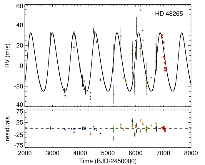
Fig. 8. Same as Fig. 2 but for system HD 48265. The literature MIKE data are shown in blue, the literature HARPS data in orange and literature CORALIE datapoints in green, while our HARPS survey data are shown in red.
