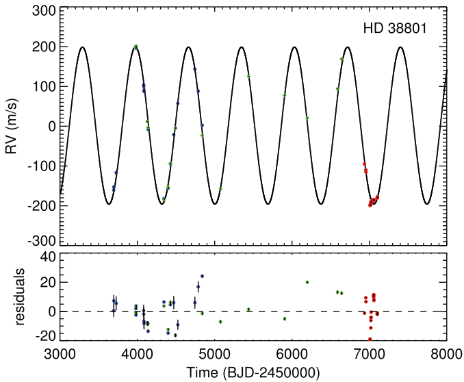
Fig. 7. Same as Fig. 2 but for system HD 38801. The literature Subaru data are shown in blue, literature Keck data in green, while our HARPS survey data are shown in red.
