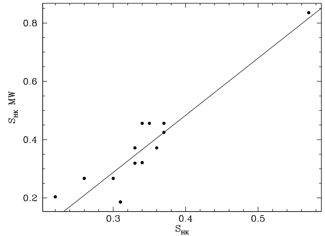
Figure A1. The S_{HK} index in the Mount Wilson scale as a function of the S_{HK} index directly measured by us for nine stars which have common TNG/HARPS-N and LAMOST low-resolution spectra.
