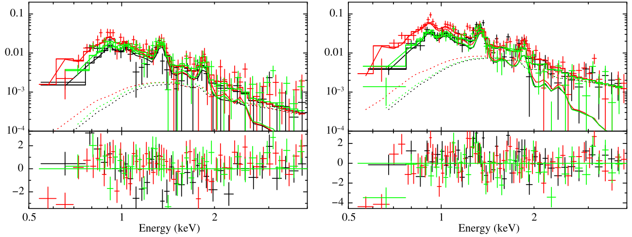
Figure 5. Background-subtracted spectra of the north (left) and south (right) regions. Black, red, and green crosses represent the XIS0, 1, and 3 spectra, respectively. Solid and dotted lines represent vnei and power-law component, respectively.
