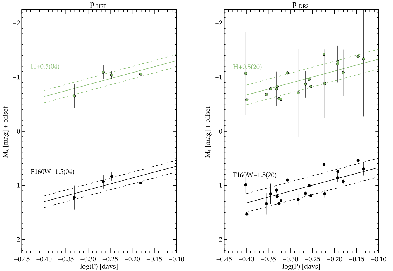
Figure 3. Period–luminosity (PL) relations for our Galactic RR Lyrae; only R Rab (fundamental pulsators) are used. The left panel consists of the four R Rab with HST /FGS parallaxes from Benedict et al. (2011), the right panel shows R Rab in the Gaia DR2 parallax sample, our F160W sample contains 20 stars (see Section 5 for a discussion of our selection method). We compare our F160W PL relation with a fit to ground-based 2MASS H -band magnitudes (Monson et al. 2017).
