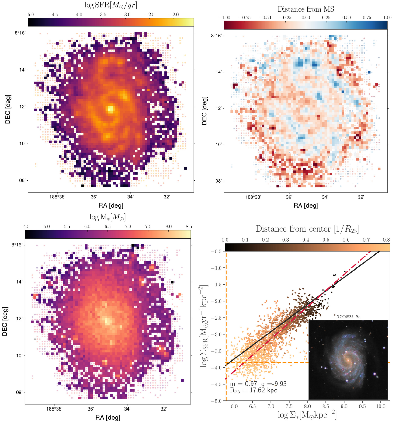
Figure A5. Same as Fig. 4, for NGC 4535.
