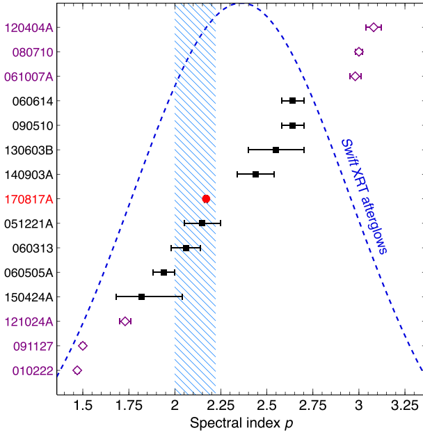
Figure 2. Spectral index p of the shock-accelerated electrons for GW 170817/GRB 170817A (filled circle) and a sample of short GRBs (filled squares) and long GRBs (open diamonds) with good afterglow constraints. The dashed line shows the distribution inferred from X-Ray Telescope (XRT) afterglows (Curran et al. 2010). The hatched area shows the range of values predicted by shock theory. Data are from Roming et al. (2006), Soderberg et al. (2006), Mundell et al. (2007), Resmi & Bhattacharya (2008), Xu et al. (2009), Krühler et al. (2009), Kumar & Barniol Duran (2010), Troja et al. (2012, 2016), Fong et al. (2015), Varela et al. (2016), and Knust et al. (2017).
