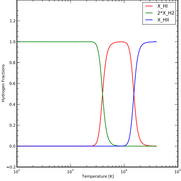
Fig. 2. Variation of different hydrogen fractions ( X_{\text{HI}} : Atomic red, X_{\text{H2}} : Molecular green and X_{\text{HII}} : Ionized blue) obtained at equilibrium with different temperatures. Note that the total sum of fractions, i.e., X_{\text{HI}} + 2.0 \cdot X_{\text{H2}} + X_{\text{HII}} is conserved.
