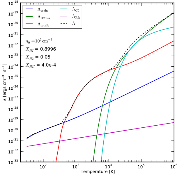
Fig. 3. The figure shows different components of radiative cooling functions with various colored lines. The values are obtained for an initial number density, n_0 = 10^5 \text{ cm}^{-3} and fractions mentioned in the figure. The sum of all the components is drawn with a black dashed line to obtain the value of \Lambda in \text{ergs cm}^{-3} \text{ s}^{-1} following Eq. 26
