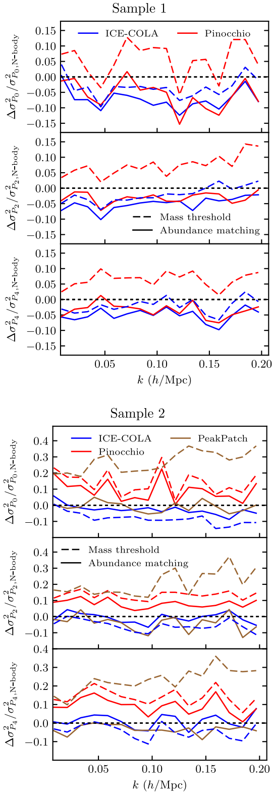
Figure A2. Relative difference of the variance of power spectrum multipoles with respect to N-body for the sample 1 (top plot) and sample 2 (bottom plot). Each plot shows monopole (top panel), quadrupole (middle panel), and hexadecapole (bottom panel) for mass samples (dashed lines) and density samples (solid lines).
