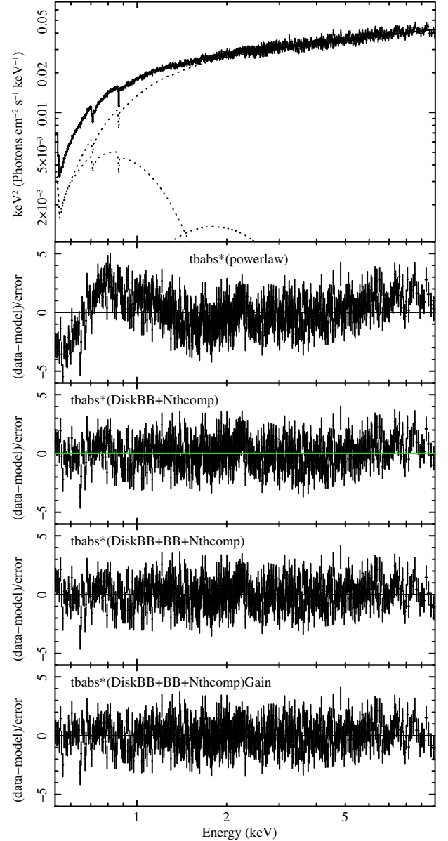
Figure 9. (Top panel) XMM-Newton EPIC-pn hard state spectrum fitted by the best-fitting model (disc blackbody plus blackbody and a dominant Comptonization components absorbed by neutral material). No signs of ionized absorption is present. (Centre top panel) Residuals once the data are fitted with an absorbed power law. (Centre panel) Residuals after fitting with an absorbed disc blackbody plus Comptonization model. (Centre bottom panel) Residuals after the addition of a blackbody component. (Bottom panel) Residuals after the consideration of a gain offset in the response files.
