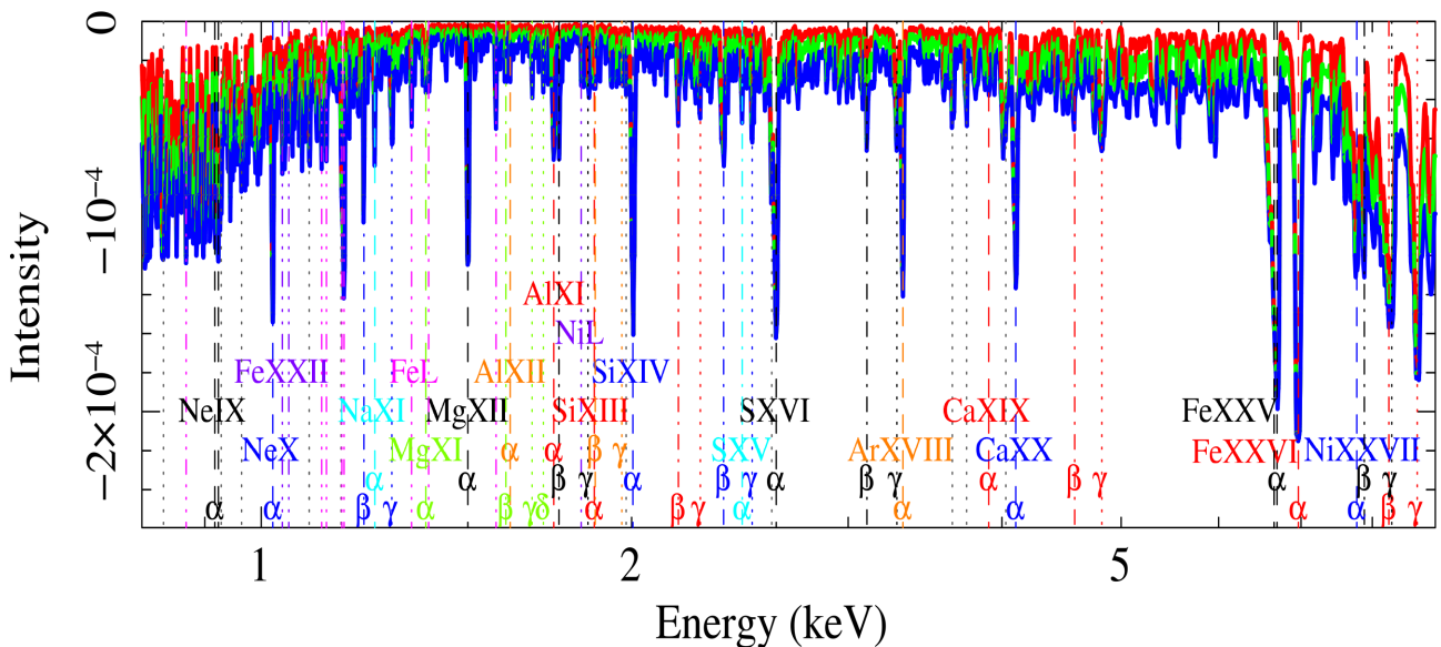
Figure 4. Residuals to the presence of narrow ( \sigma = 1 eV) absorption lines in the Chandra HETG (HEG + MEG) spectra. The red, green, and blue solid lines show the 68, 90, and 99 percent confidence contours. 60 absorption lines are detected. We highlight with a vertical line each detected absorption feature. The same colour is used for features associated to the same series. In particular, the energies of the \alpha , \beta , and \gamma transitions are reported with dashed, dash-dotted, and dotted lines, respectively. Absorption lines associated with Fe L features are highlighted with magenta dot-dot-dot-dashed lines (in violet is the density sensitive Fe XXII doublet). Unidentified lines are shown with grey dotted lines.
