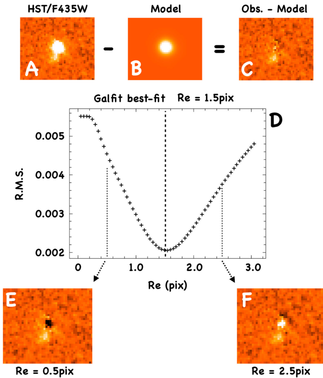
Figure 5. GALFIT modeling of the Ion2 galaxy in the F435W band (1000 Å rest-frame). In panel (C), the residuals of the observed (A)-model (B) are shown for the best-fit case ( R_e = 1.5 px \simeq 340 pc). Bottom panels show an example of two “bad” solutions (observed-model), in which positive/negative residuals are evident (panels (E)/(F)). Middle panel (D) shows the behavior of the rms calculated at the “A” position by running GALFIT in a grid of effective radii (as described in Vanzella et al. 2015). A good convergence is reached at R_e = 1.5 \pm 0.1 px. This illustrates that the source is spatially resolved at 1000 Å rest-frame. The size of the thumbnails is 1''.2 \times 1''.0 .
