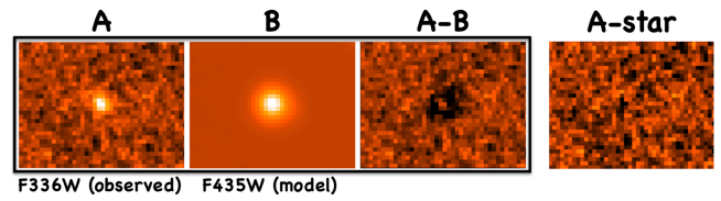
Figure 4. Difference between the observed F336W image (A) GALFIT best-fit model calculated in the F435W image (B) is shown in the right (A-B). Model A is scaled to the flux peak of the F336W source (B). This comparison suggests that the LyC emitting region is more compact than the resolved emission measured in the F435W band. In the right panel, the residuals after subtracting a star rescaled to the source flux are shown. The size of the thumbnails is 1''.2 \times 1''.0 .
