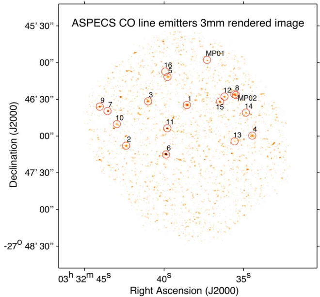
Figure 1. Rendered CO image toward the HUDF, obtained by coadding the individual average CO line maps around the 16 bright CO-selected galaxies and the 2 lower significance MUSE-based CO sources (labeled MP). Regions with significances below 2.5\sigma in each of the average maps are masked out prior to combination. The location of these individual detections is highlighted by solid circles and their IDs. The tendency of sources to lie in the top two-thirds of the map is likely a combination of clustering and chance, given the sensitivity of the observations is fairly uniform across this region. We note that in this representation of the combined CO map, some individual images might have larger weight (lower noise) than others, and thus some noise peaks might appear as brighter than other statistically significant sources.
