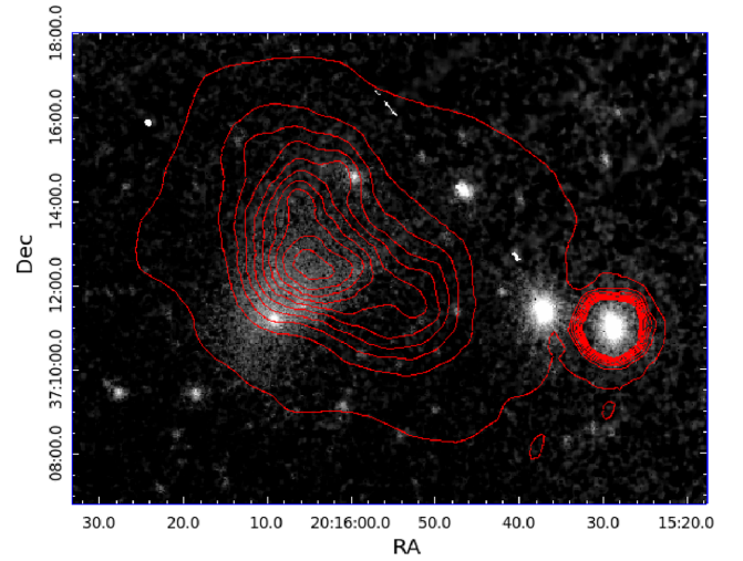
Figure 7. Merged MOS1, MOS2, and pn image overlaid with the radio contours from the Dominion Radio Astrophysical Observatory as part of the Canadian Galactic Plane Survey (Taylor et al. 2003).
