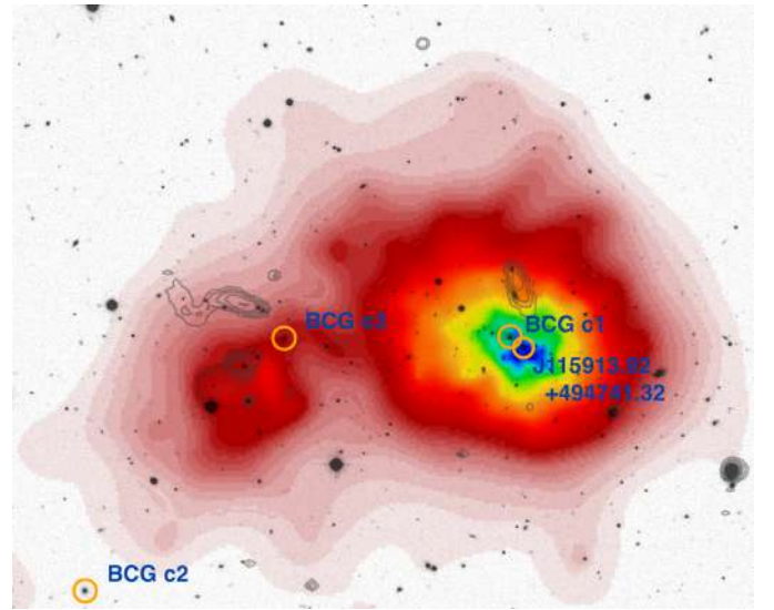
Fig. 5. Colourscale: Chandra X-ray surface brightness distribution with point sources subtracted and adaptively smoothed. Grey contours: LOFAR high-resolution image (using Briggs weighting –1.0) to indicate the positions of the radio galaxies. Greyscale: SDSS r -band image. The positions of the three initial BCG candidates c1, c2, and c3 at J115914.85+494748.1, J115943.99+494459.6, and J115930.36+494747.4, respectively, and the bright galaxy close to the X-ray peak are highlighted with orange circles (see Sect. 4.4).
