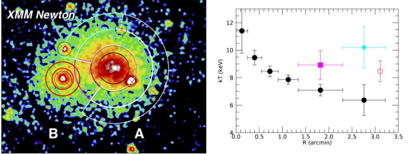
Fig. 4. Left: X-ray surface distribution as obtained from XMM-Newton in the band 0.7–1.2 keV, smoothed with a Gaussian with a width of 12''. The two subcomponents of A1430 are clearly visible. Annuli and sectors show the regions used for spectral extraction and analysis, while barred circles indicate the point sources excluded from the analysis. The labels ‘A’ and ‘B’ denote the main component and the subcomponent of the cluster, respectively. Right: temperature distribution in the cluster. Filled black circles show the temperature profile of the main cluster, measured in the black and white marked regions in the left panel which exclude the interaction with the subcomponent. The magenta and cyan regions show the temperature in the sectors marked with the same colours in the left panel, while the red empty circle represents the temperature of subcomponent A.
