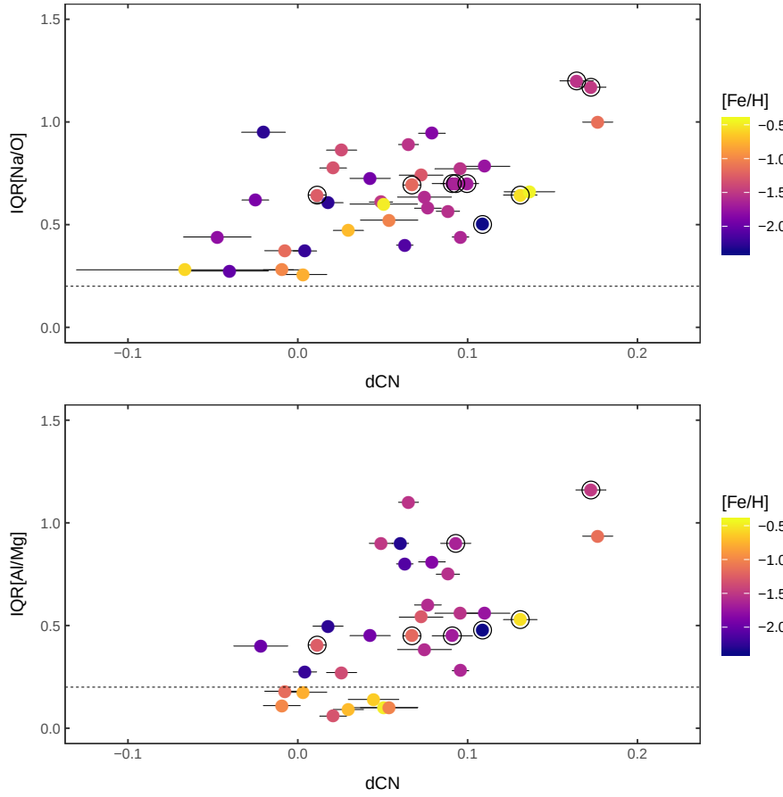
Fig. 5 Upper panel: run of the interquartile \text{IQR}[\text{Na}/\text{O}] of the distribution of [\text{Na}/\text{O}] abundance ratios within a cluster (see compilation in Appendix 1) and the spread in CN as derived from the spread in UV colours along the RGB \mathcal{A}_{F275W, F336W, F438W} from Milone et al. (2017a). Lower panel: the same, but for the interquartile \text{IQR}[\text{Al}/\text{Mg}] of [\text{Al}/\text{Mg}] abundance ratios. Circled dots are for Type II clusters according to the classification by Milone et al. (2017a). In both panels, points below the dashed lines are actually consistent with no spread at all because they corresponds to the observational errors. Colours code metallicity (see scale on the right of the plot)
