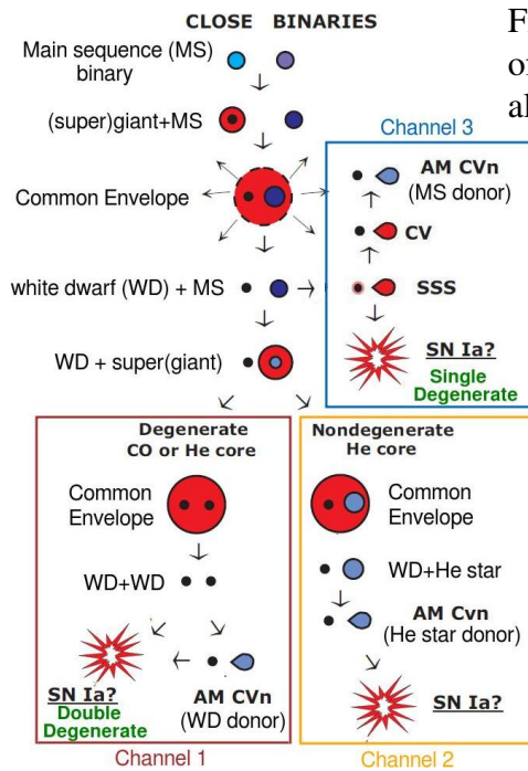
Figure 1: Evolution of close binary, resulting in mergers or systems with high- (SSSs) and low accretion rates (CVs and AM CVns).
